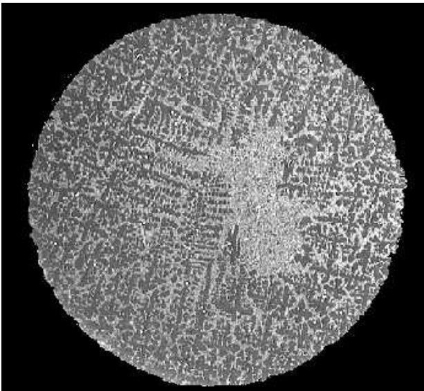
Figure 9 - Cross section through an A357 sample solidified with RMF at 6 mT. Slightly of center is an area free of dendrite. This zone exhibits a eutectic microstructure only.
