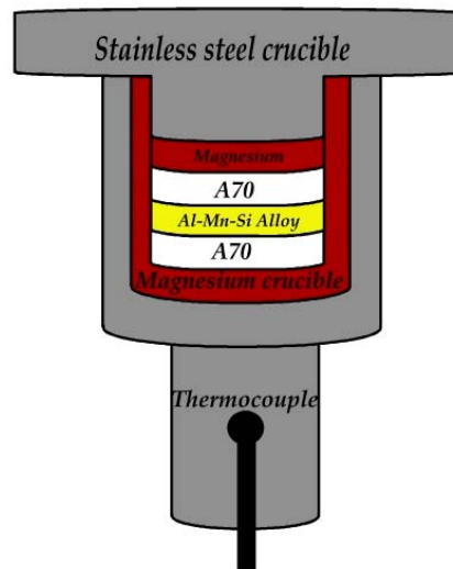
Figure VI-3: A cross-section of the experimental set-up. The stainless steel cylinder is placed onto the thermocouple.
