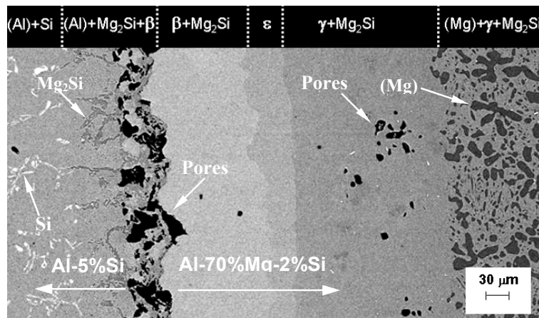
Figure 3 – SEM micrograph showing the junction of the diffusion couple after 7 months at 300 °C (backscattered electron imaging).
