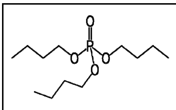
Figure 8 : Configuration du Tributylphosphate
