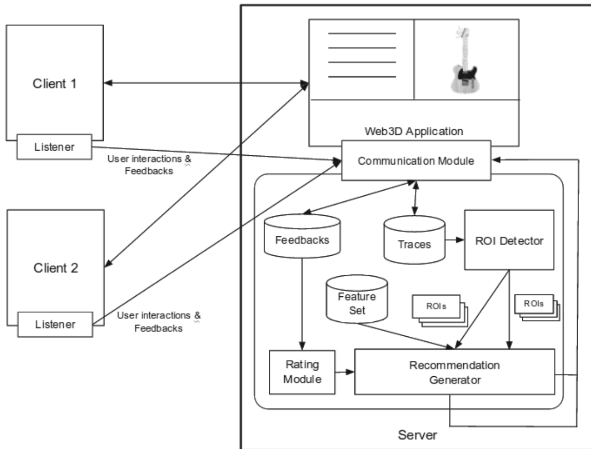
Figure 3.26: System Architecture.
