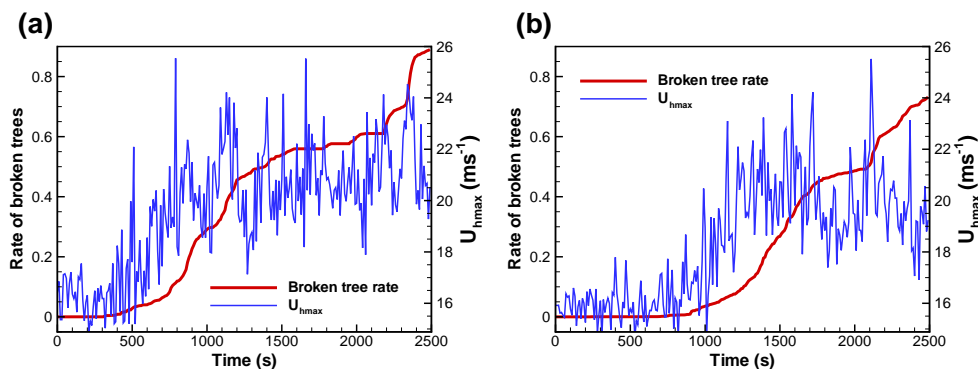
FIGURE 3.11 – Time series of the rate of broken trees (red solid line) and canopy top maximum wind velocity (solid blue line) as simulated in cases 7 (a) and 7* (b) with two different initial wind gust timing.
