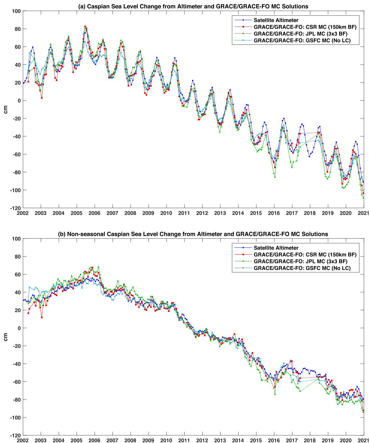
Fig. 6. (a) Monthly CSL from altimetry and the three MC solutions for April 2002–December 2020. The CSR series adds signals from a 150-km BF to reduce leakage. The JPL solutions are corrected for signal leakage by adding signals from all 3 \times 3 degree elements overlapping the Caspian Sea (noted as 3 \times 3 BF). TWS contributions are removed from the BF zones using the GLDAS model as described in the text. The 1-year gaps between GRACE and GRACE-FO are connected by dashed lines (b) similar to (a), but with annual and semiannual variations removed from all-time series.
