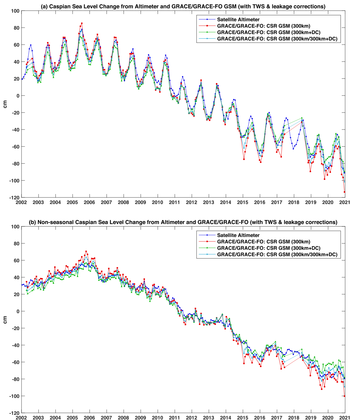
Fig. 4. (a) Monthly CSL from satellite altimetry and CSR GSM estimates corrected using the revised SF method that includes TWS effects (from GLDAS Noah V2.1). GSM estimates include 300-km Gaussian filtering with and without DC filtering, and the average of the two (300 km/300 km + DC). Gaps between GRACE and GRACE-FO series are connected by dashed lines. (b) Is similar to (a), but with annual and semiannual variations removed from all series. Table II gives amplitudes and phases of seasonal terms that have been removed.
