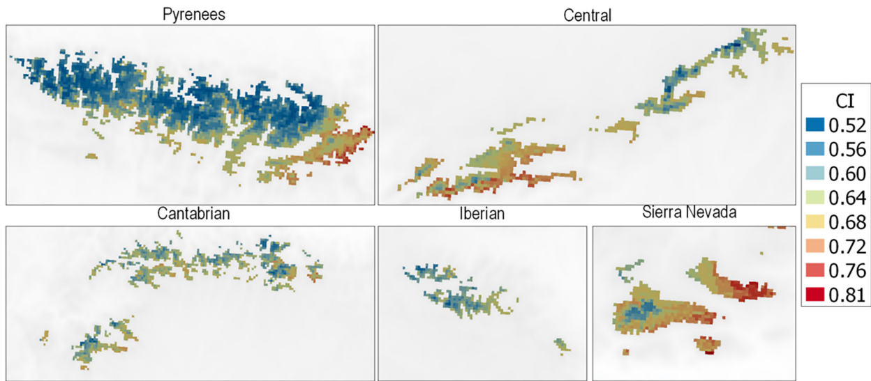
FIGURE 3 Spatial distribution of the concentration index through the Iberian Peninsula Mountain ranges. [Colour figure can be viewed at wileyonlinelibrary.com ]
