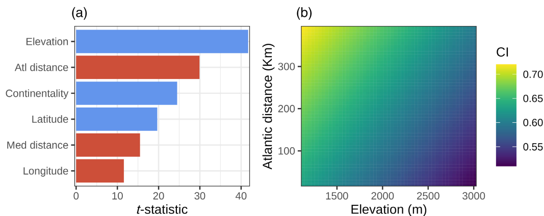
FIGURE 8 Partial dependence analysis of the concentration index (CI) and the geographical predictor variables. (a) t -Statistic performance of the geographical variables included in the model. Blue and red colours show an inverse or direct relationship between CI and the geographical factors, respectively. (b) Relationship between Atlantic distance and elevation. The colour gradient indicates the values of the CI with respect to these two variables. [Colour figure can be viewed at wileyonlinelibrary.com ]
