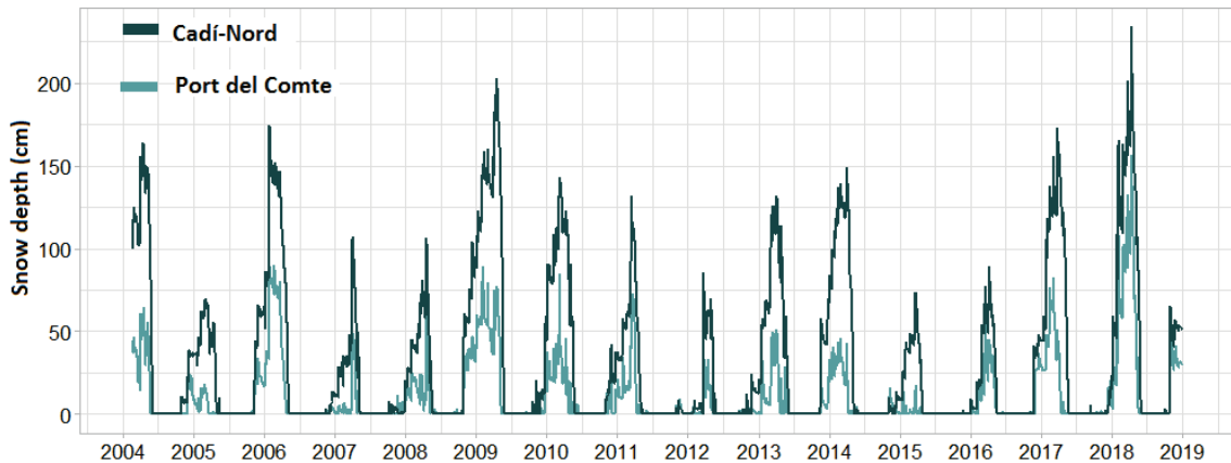
Figure 4. Annual evolution of snow depth (cm) at Cadí-Nord and Port del Comte.
