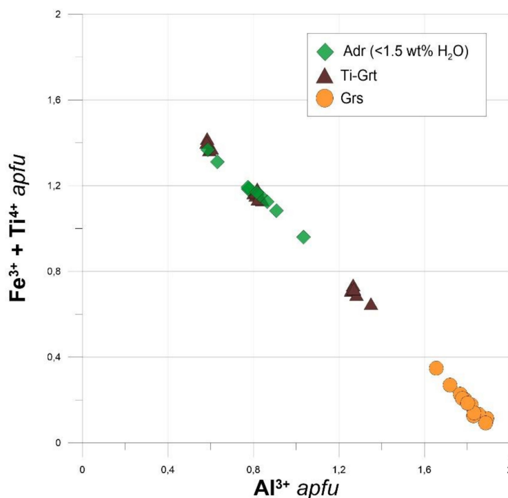
Figure 9. Garnet solid solution chemistry characterized by negative correlation between Al^{3+} and Fe^{3+} + Ti^{4+} at Y crystallographic site.
