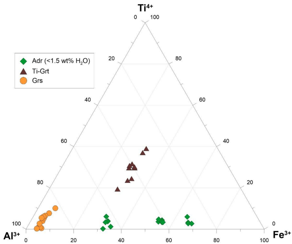
Figure 5. Chemical variations of the garnet solid solution projected into Fe^{3+} -Ti-Al ternary diagram. The low hydrated ADR group represents younger rims of otherwise hydrated garnet cores.
