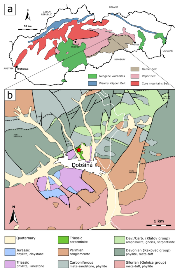
Figure 1. (a) Geological sketch map of the Western Carpathians in Slovakia; (b) Simplified geological map of Dobšiná region (modified after [29]). The red star denotes the rodingite occurrence.
