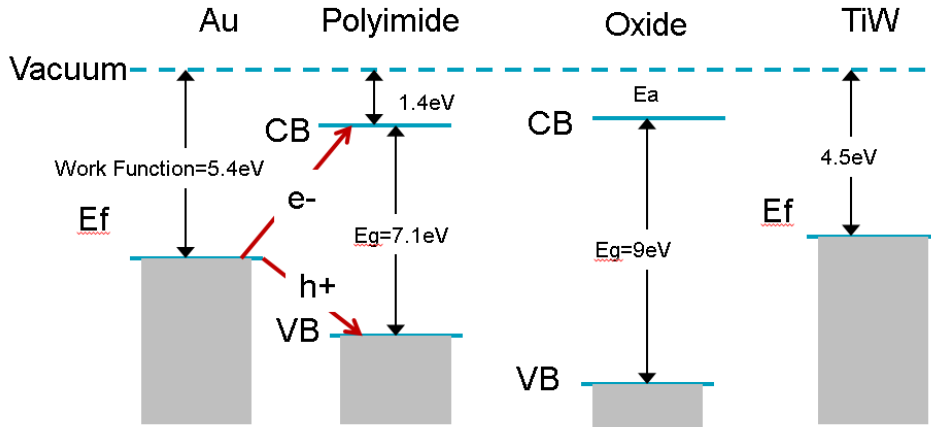
Figure 14. Band diagram for charge injection
