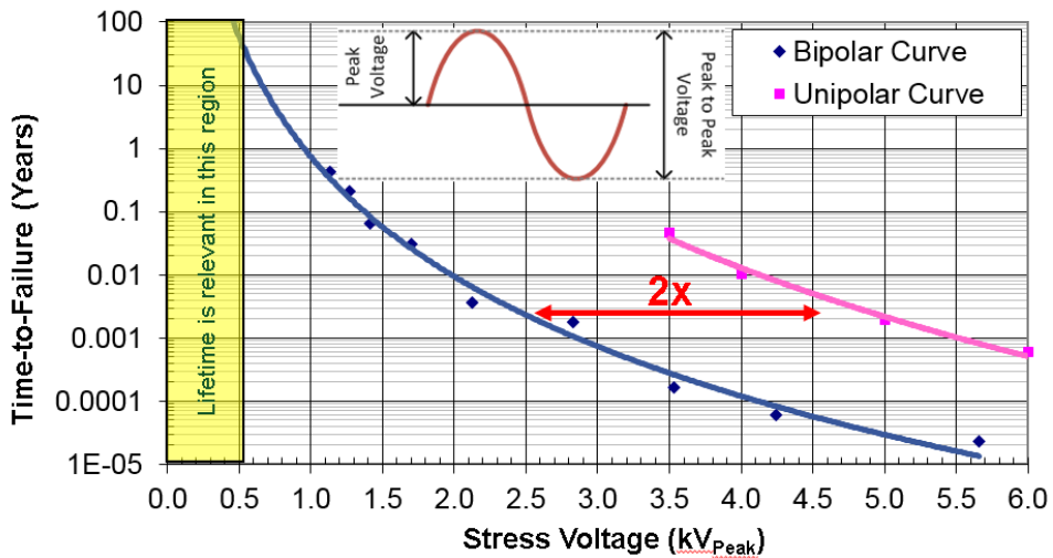
Figure 12. Time to failure comparisons for AC bipolar vs Uni-polar
