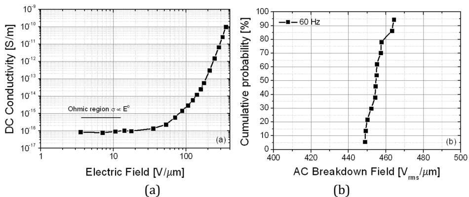
Figure 6. Main intrinsic electrical properties of spin-coated polyimide films measured at wafer level: (a) DC conductivity vs. electric field and (b) AC breakdown field distribution.
