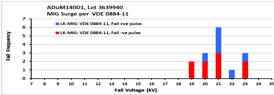
Figure 7. Surge performance for isolators with polyimide films 30 μm-thick
