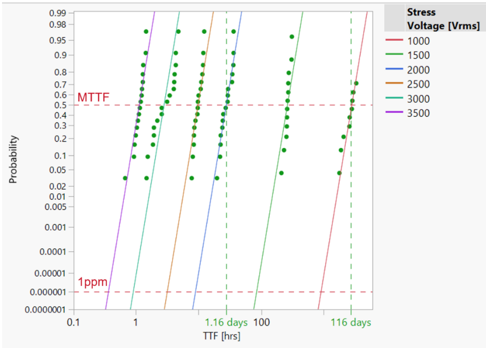
Figure 9. Weibull distribution for isolators with 20 μm thick polyimide
