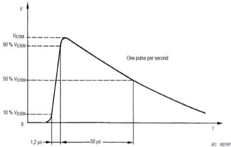
Figure 5. IEC61010-1 Surge test waveform
