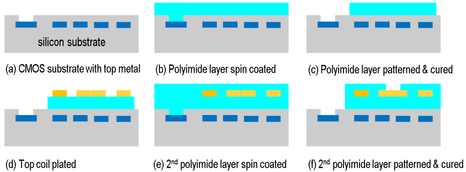
Figure 3. Isolation transformer process flow
