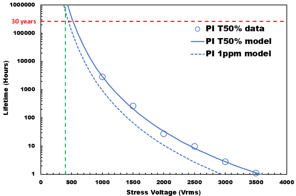
Figure 10. Time to failure plot for isolators with 20 μm thick polyimide
