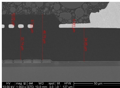
Figure 4. Cross-section for the fabricated isolation transformer
