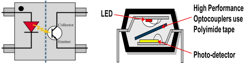
Figure 1. (a) Opto-coupler schematic (b) Opto-coupler package cross-section
