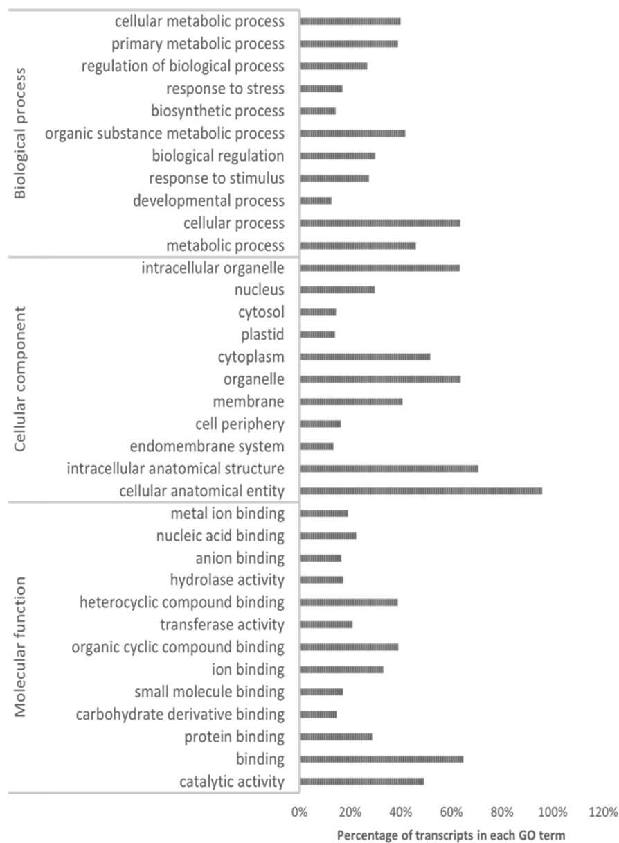
Figure 2. The GO classification of H. incana transcripts in response to Pb stress.
