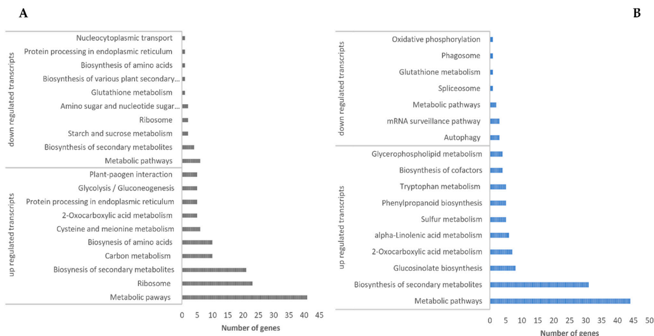
Figure 5. Top pathways of DEGs in roots (A) and aboveground parts (B) of H. incana in response to Pb exposure.
