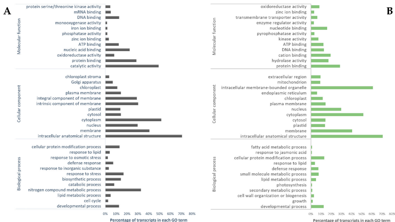
Figure 4. Top 12 GO classification of upregulated genes in roots (A) and aboveground parts (B) of H. incana under Pb exposure.
