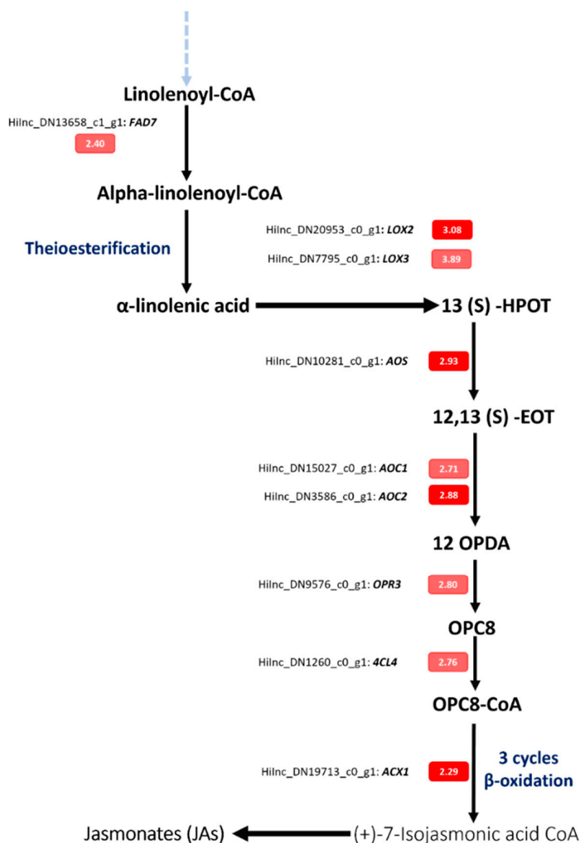
Figure 6. Expression level of genes implicated in the JAs biosynthesis pathways in H. incana under Pb exposure. The red color represents the genes selected using the restrictive method “Bonferroni”, and the light red represent the genes selected without using the restrictive method.
