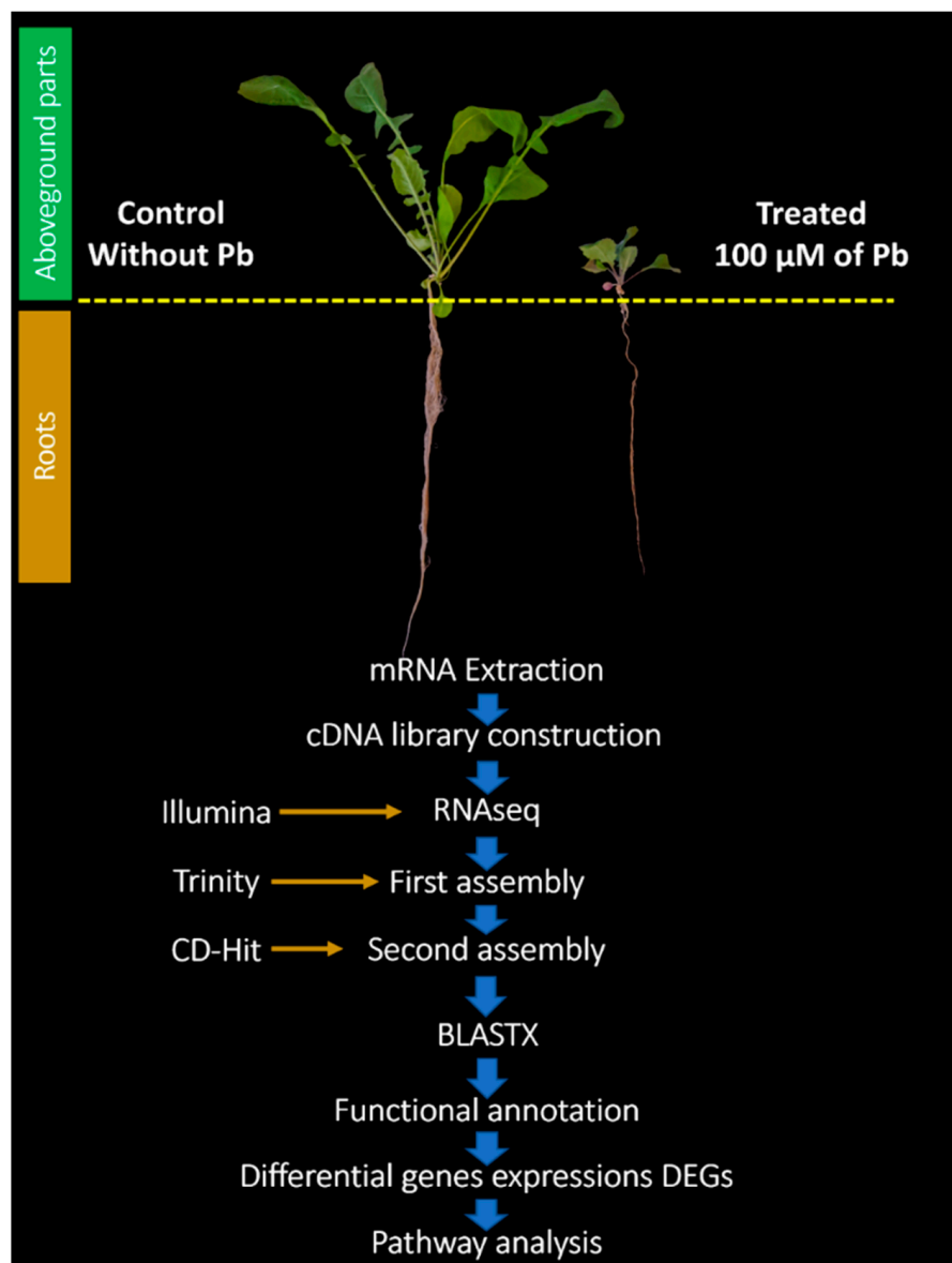
Figure 1. Experimental design for RNAseq and pipeline.
