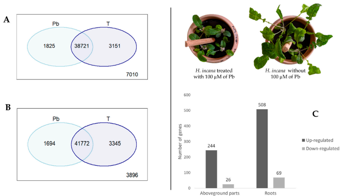
Figure 3. Venn diagram and DEGs in roots and aboveground parts of H. incana : (A) Venn diagram for control (T) and treated (Pb) in aboveground parts; (B) Venn diagram for control (T) and treated (Pb) in roots; and (C) number of DEGs in different tissues.
