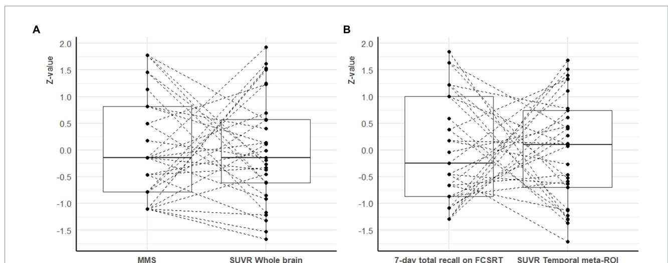
FIGURE 1 Inter-individual heterogeneity of the relationship between cognitive performances and SUVR values. (Panel A) represents the relationship between the MMS score and the whole brain SUVR. (Panel B) shows the relationship between the 7-day total recall on the FCSRT and the temporal meta-ROI SUVR. To facilitate comparisons between the distribution of cognitive scores and SUVR values, we calculated z-scores based on the present population (i.e., a null z-value corresponds to the mean of the study cohort). Each line represents one AD patient (MAB or HAB). The reference region was the CC for the whole brain SUVR (panel A) and the WB for the temporal meta-ROI (panel B). CC: cerebellar cortex; FCSRT: free and cued selective reminding test; MMS: mini-mental state examination; ROI: region of interest; SUVR: standard uptake value ratio; WB: whole brain.
