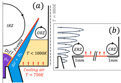
Fig. 9. Proposed flame topology — (a) Global view, (b) Zoom on the chamber bottom.
