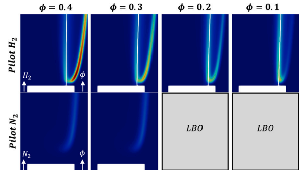
Fig. 13. Instantaneous views of the hydrogen source term for equivalence ratio of the premixed side varying from \phi = 0.4 to 0.1 (columns) with H_2 as pilot injection (top) and N_2 (bottom) - Stoichiometric line (white).
