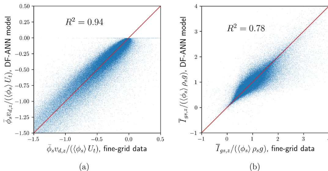
Figure 7. Assessment of the DF-ANN model predictions on (a) the drift flux and (b) the filtered drag force using explicit eq 15 with the scalar variance-based 4-marker model ( \bar{\phi}_s , \bar{\Delta} , \tilde{u}_{slip,z} , \phi_s^{\prime 2} ).
