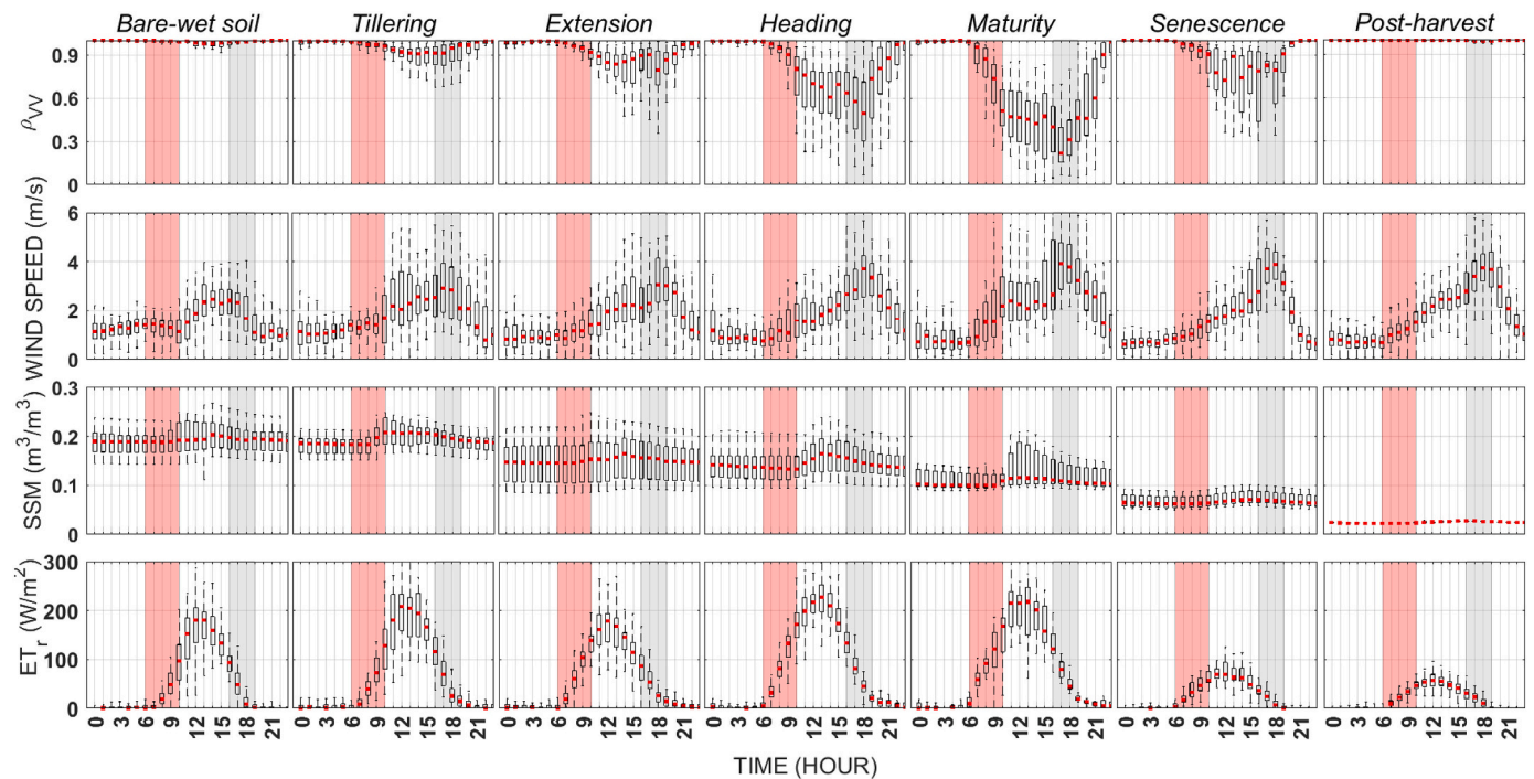
Fig. 4. Diurnal cycles represented by boxplots (median is indicated in red, the box bottom edge indicate the 25th percentiles and the box top edge show the 75th percentiles) of \rho_{VV} with 15-min baseline, wind speed, SSM and LE for 7 different sub-periods of the wheat season (see text). The morning decrease and evening increase of \rho_{VV} are shaded in red and gray, respectively. (For interpretation of the references to colour in this figure legend, the reader is referred to the web version of this article.)
