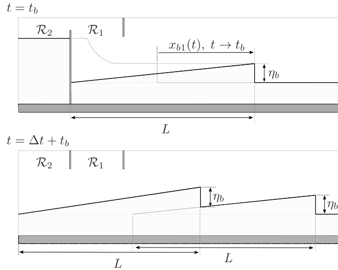
Fig. 6. Sketch of the model described in Section 5.2, corresponding to two bores generated by the same volume of fluid ( h_1 = h_2 \equiv h ; l_1 = l_2 \equiv l ) in \mathcal{R}_1 and \mathcal{R}_2 . At t = t_b , the evolving front x_{b1} , following Stoker's solution of an initial column collapse over a constant fluid layer depth h_0 (dotted line), has spread over a distance balancing the volume of \mathcal{R}_1 and a bore wave model of length L and front height \eta_b . This is referred to as the fully developed wave. At t = \Delta t + t_b , the second bore emanating from \mathcal{R}_2 is fully developed and evolves on the tail of the preceding one.
