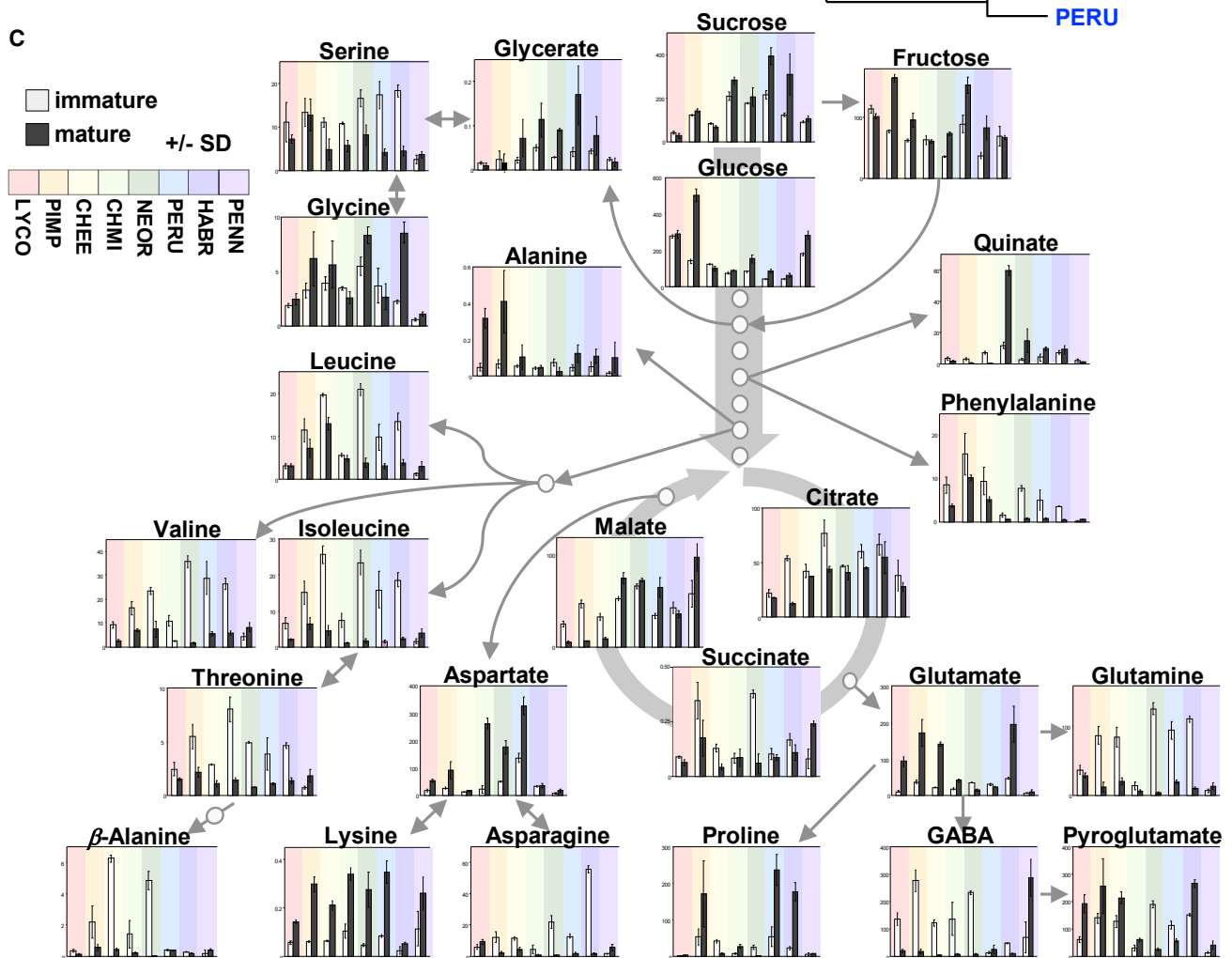
Figure 2. Metabolomic Signatures Defining Fruit Ripening in Diverse Tomato Species.
