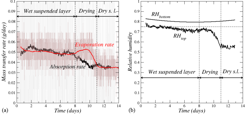
FIG. 6. Salt experiment: (a) Comparison of absorption and evaporation rates; (b) computed evolutions of relative humidity at suspended layer top and bottom surfaces.
