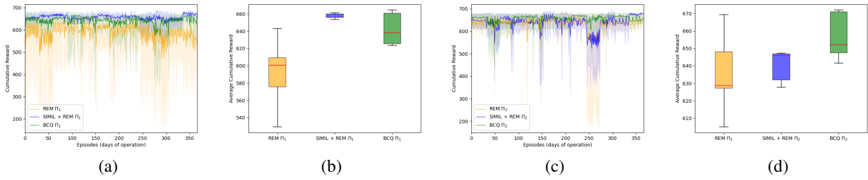
Figure 1: (a) and (c) are respectively the min, max, and average cumulative reward for the set of policies \Pi_1 and \Pi_2 . (b) and (d) shows the average of the cumulative rewards along with the episodes for \Pi_1 and \Pi_2 .
