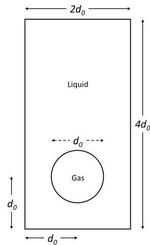
Figure A1. Physical domain and initial configuration for a verification test case.
