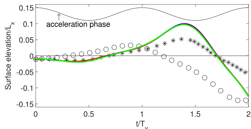
(b) Inverted acceleration phase
