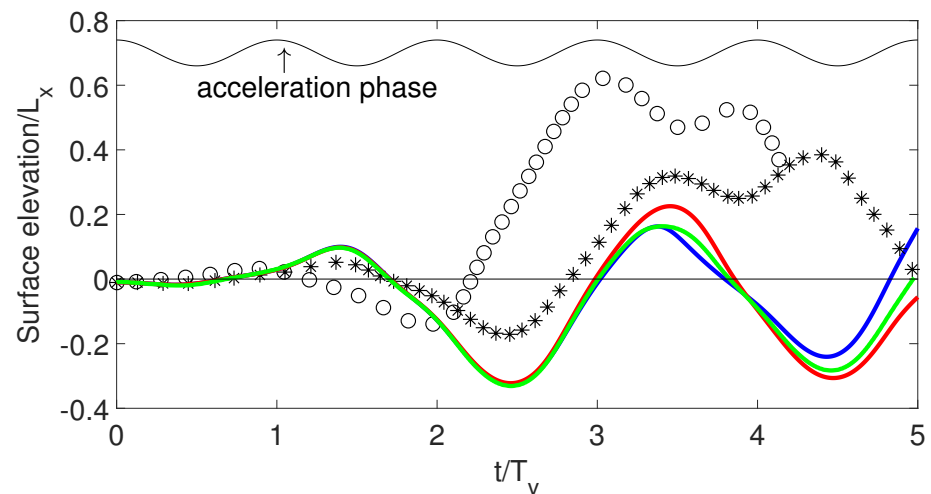
Figure 4. Comparison of different approaches in the nonlinear regime: surface elevation at the midpoint-inverted acceleration phase. (o) Wright et al. [7], (*) PF_S [15], (—) EbFVM_S (this work), (—) FT_S (this work), (—) VOF_S (this work).
