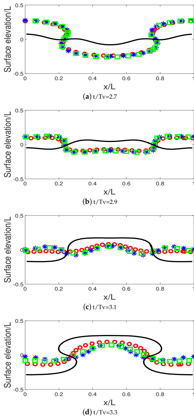
Figure 6. Comparison of the interface shape evolution—Nonlinear case with inverted acceleration. (—) PF_S [15], (○) FT_S (this work), (*) EbFVM_S (this work), (□) VOF_S (this work).
