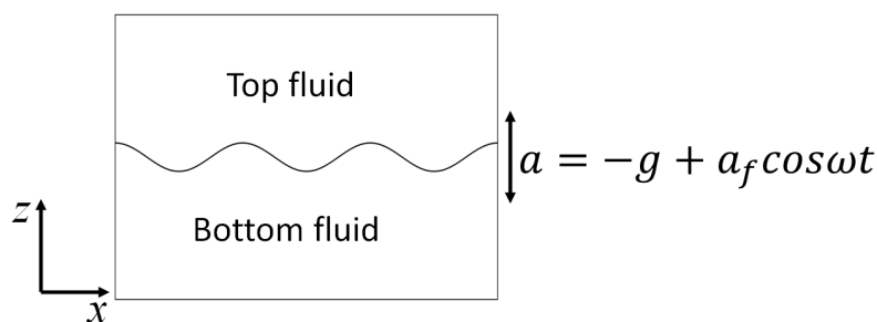
Figure 1. Schematic distribution of fluids in the two-dimensional container.
