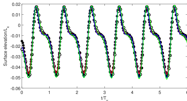
(b) k = 73 \text{ mm}^{-1} (harmonic case)
