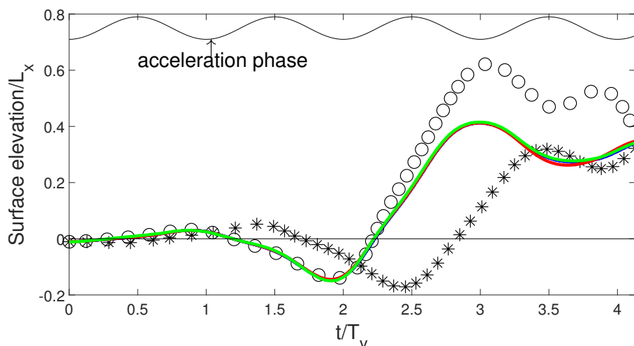
Figure 3. Comparison of different approaches in the nonlinear regime: surface elevation at the midpoint. (o) Wright et al. [7], (*) PF_S [15], (—) EbFVM_S (this work), (—) FT_S (this work), (—) VOF_S (this work).
