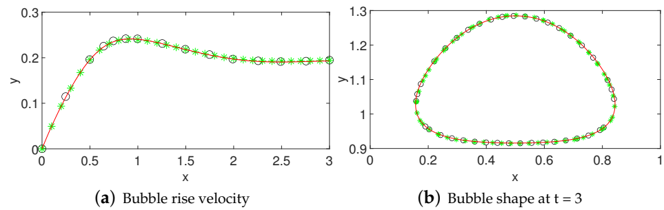
Figure A2. Verification test: Rise velocity and bubble shape for test case 1 of Hysing et al. [33] (o) TP2D [33], (*) VOF_S (this work), (–) FT_S (this work).
