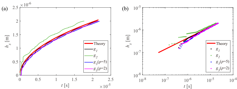
Fig. 3. Evolutions of solidification front for cases with different g functions compared to the exact solution given by relation 29. (a) a linear plot, (b) a log-log plot.
