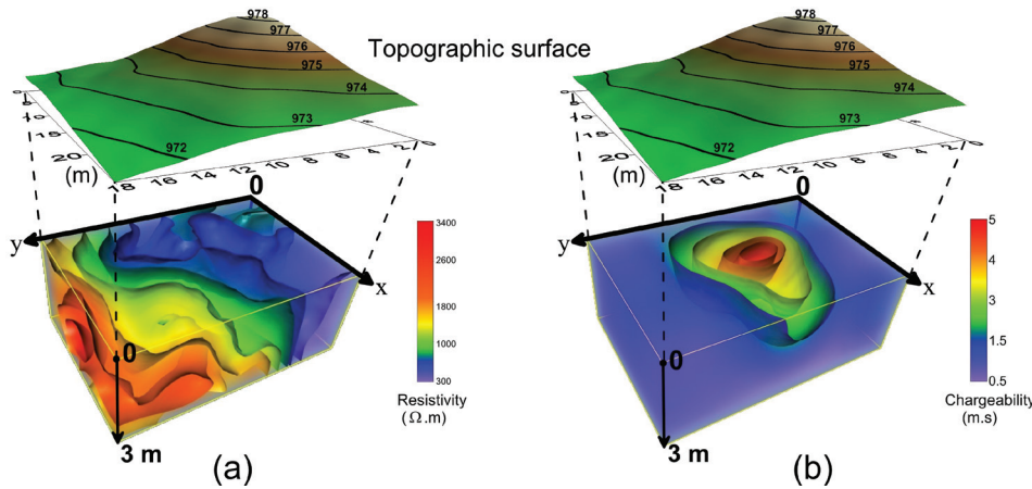
FIGURE 4 3D tomography of the slag heap in volume: (a) resistivity and (b) chargeability. The height of the topography with respect to the 3D structure is not to scale.
