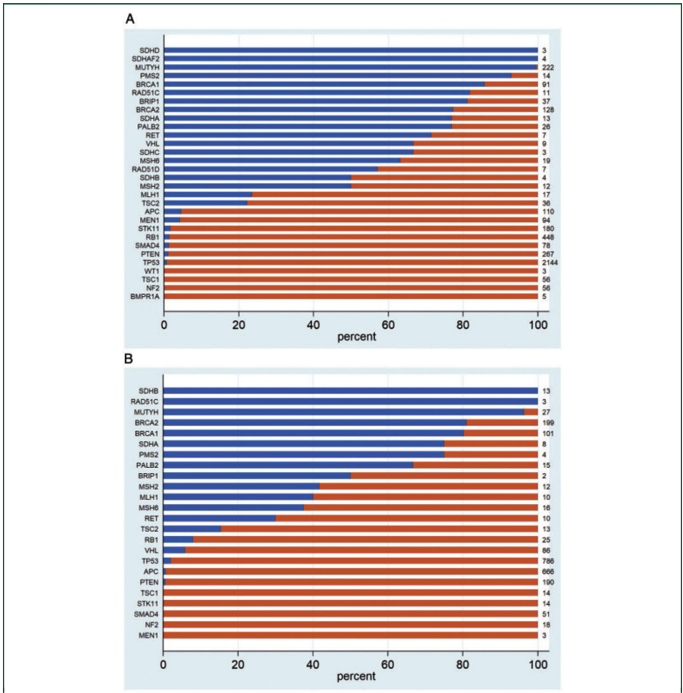
Figure 3. Distribution of germline and somatic pathogenic variants detected upon tumour analysis for 30 high-actionability CSGs. (A) Off-tumour and (B) on-tumour.
