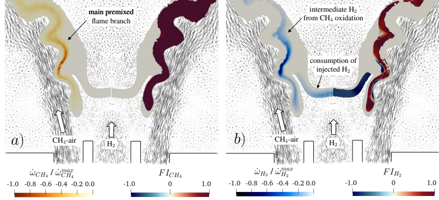
Fig. 4: Instantaneous axial cut of the PH10 case showing on the left the source term of CH 4 (a) and H 2 (b) conditioned by the heat release rate and on the right the associated Takeno index. The background of the images evidences the premixed CH 4 -air mixture and the H 2 stream exiting the coaxial injector.
