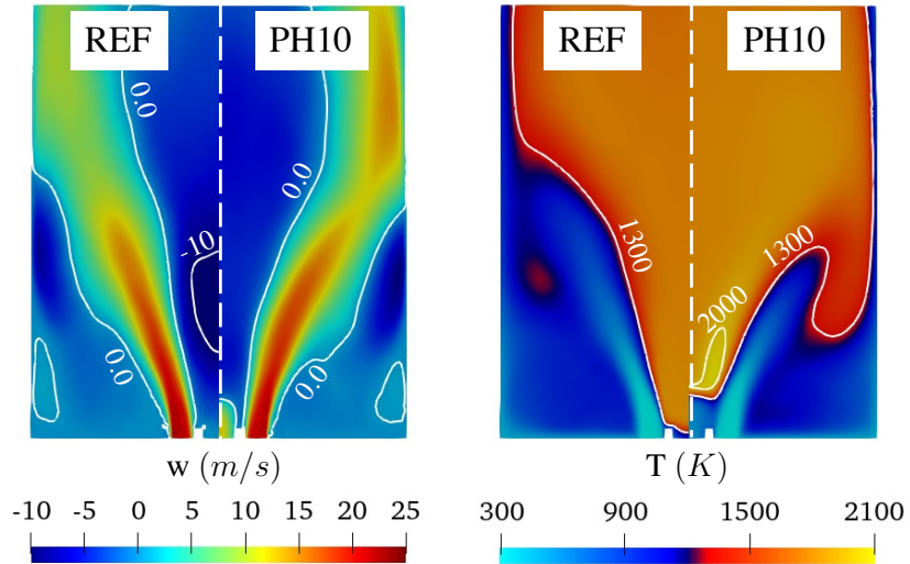
Fig. 3: Comparison of time-averaged numerical results for REF and PH10 in terms of axial velocity (a) and mean temperature (b) for unforced conditions.
