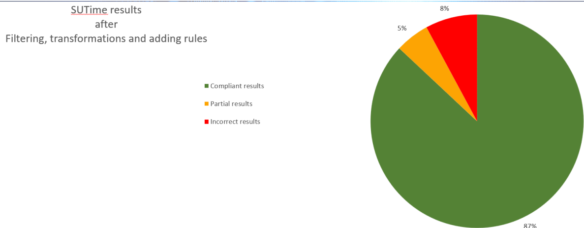
[Fig.10 – Evaluation of modified SUTime performance]
