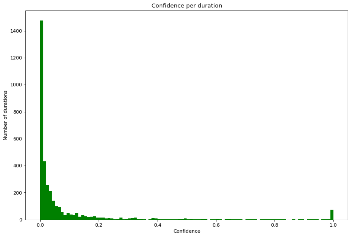
[Fig.17 – Histogram of entity association confidence index distribution]
