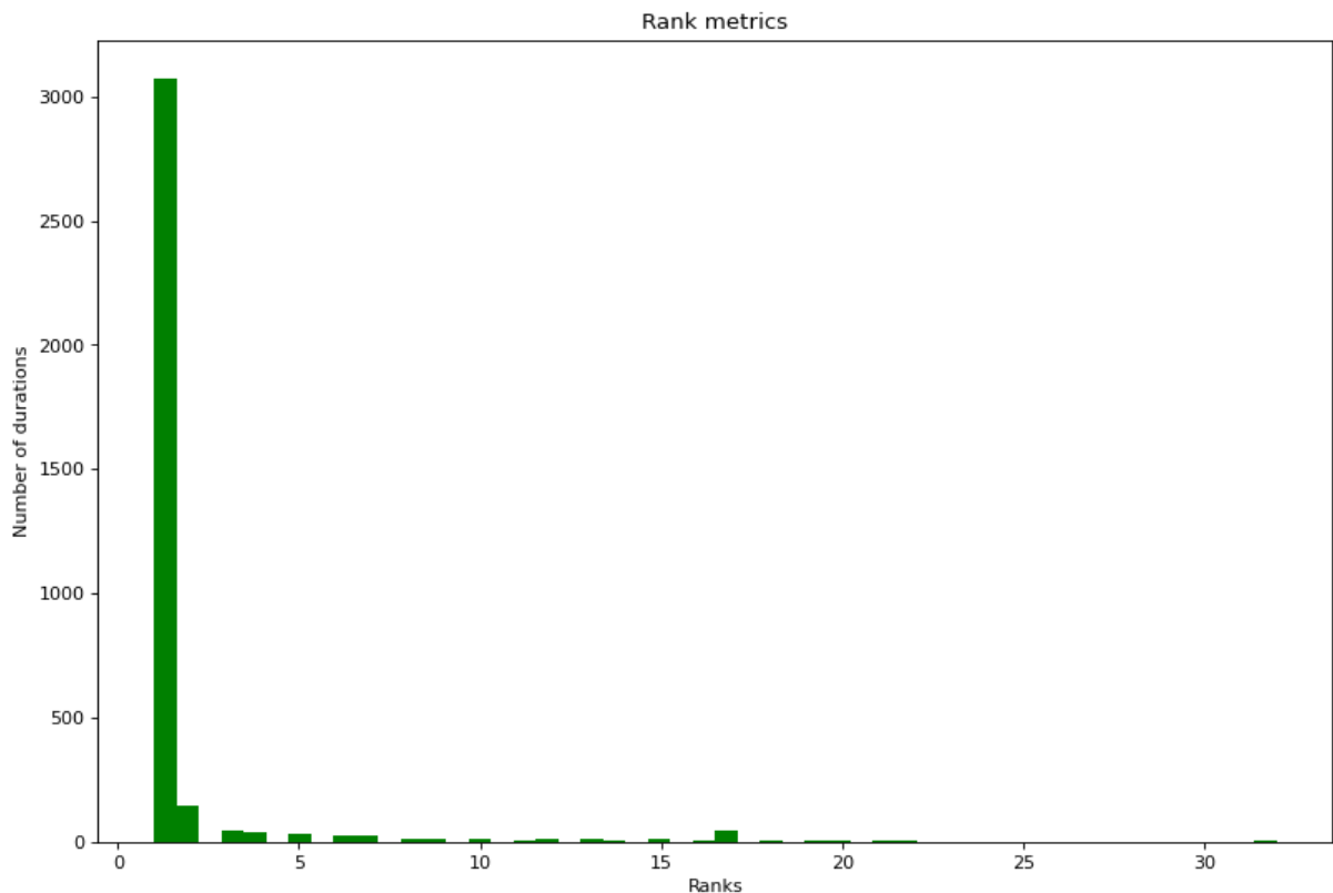
[Fig.16 – Histogram of time interval rank distribution]
