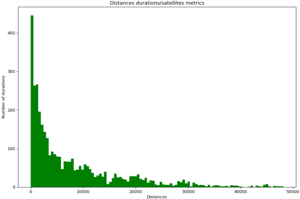
[Fig.14 – Histogram of interval/satellite distance distribution]
