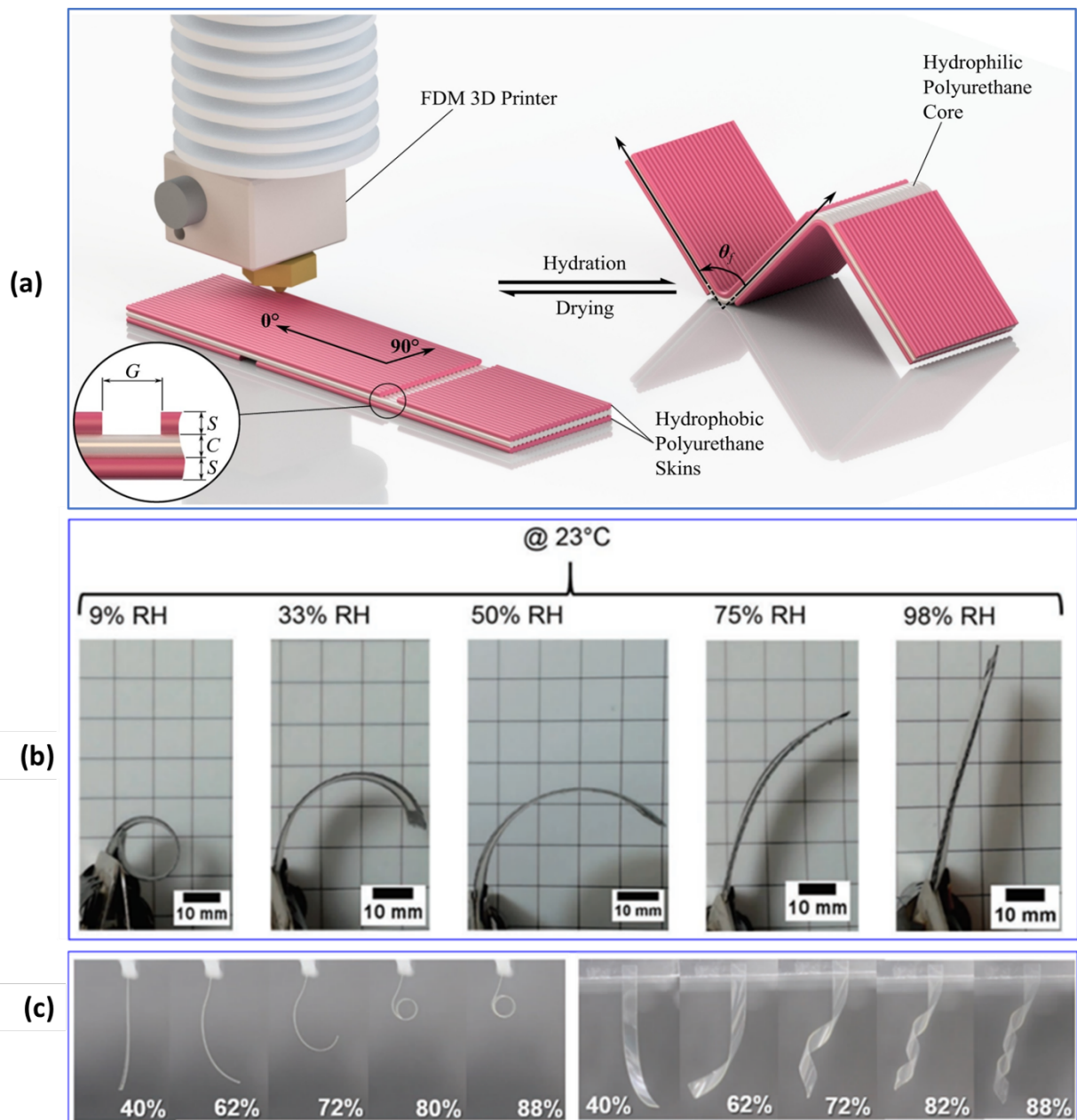
Figure 14. a. 3D-printing of self-folding multi-materials moisture-responsive structure [223]. Copyright 2019, Elsevier. b. Shape evolution of 3D printed sample made from Polyamide and carbon fibers with humidity increase [22]. Reproduced with permission. Copyright 2019, Wiley. c. Shape evolution of liquid crystal elastomer parts under different humidity conditions. Reproduced with permission. [224] Copyright, Wiley.
