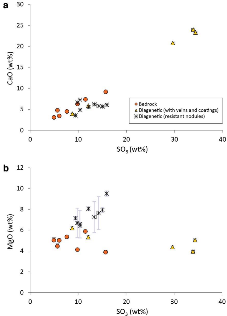
Extended Data Fig. 6: APXS data bedrock and diagenetic features. CaO ( a ) and MgO ( b ) versus SO 3 content for bedrock and diagenetic features in the investigated section. Resistant nodules, forming collectively nodular bedrock, show MgO and SO 3 enrichment. The data only includes relatively clean, dust-free targets. List of target names for bedrock: Gourdon, Bardou_DRT, Ribagnac_DRT, Chenaud_DRT, Monpazier, Plaisance_DRT, Monsec_DRT. For veins/coating: Terrasson_Lavilledieu, Festalemps_DRT, Quinsac, Biras, Pezuls. For resistant bedrock: Gardonne_DRT, Simeyrols, Rouffignac, Bosset, Bosset_offset, Nabirat, Sarlande, Salagnac, Le_Bugue.
