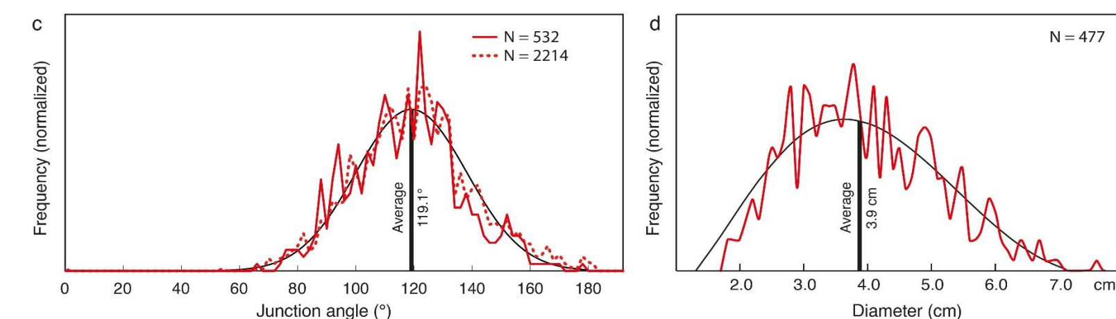
Extended Data Fig. 4: Polygonal ridges pattern analysis. Top view of bedrock from sol 3154 generated using OnSight, with circles representing marked polygon sizes (blue) and junctions (yellow dots) connected to well-expressed (solid lines) and uncertain ridges (dashed lines) forming the pattern mapped on image (a). Red contour represents the area covered on Fig. 1e, and white rectangles areas for polygon size statistics (Extended Data Table 1). Top view with extended context shows the area of analysis along with the location of closeups where polygonal ridges are observed in the distance (b). Elevation change is indicated by 1 m contour lines (yellow) to estimate the thickness of the observable strata from this location. Distribution of junction angles for well-expressed ridges only (solid red) and all ridges (dashed red) with gaussian fit (c). Distribution of polygon sizes and fit with Poisson probability distribution (d), see Extended Data Table 1.
