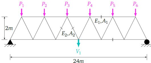
Figure 4: Truss test case: illustration (Source: Lelievre (2018))
