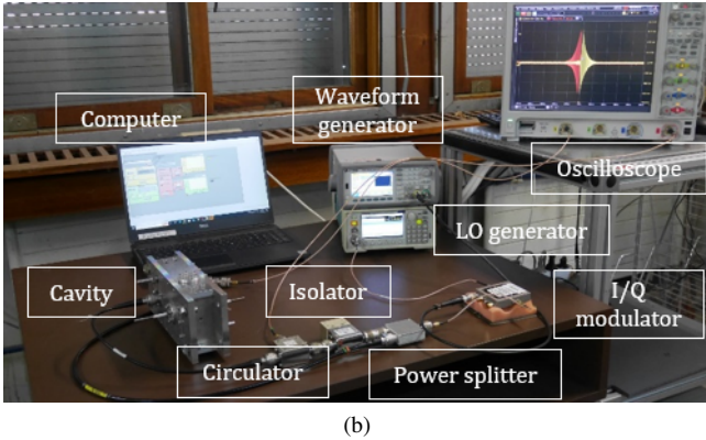
FIG. 6: (a) Scheme and (b) photograph of the experimental set-up.
