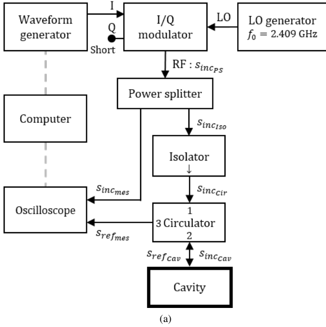
FIG. 7: Observation of a zero of the S-matrix of our cavity through our practical set-up.
