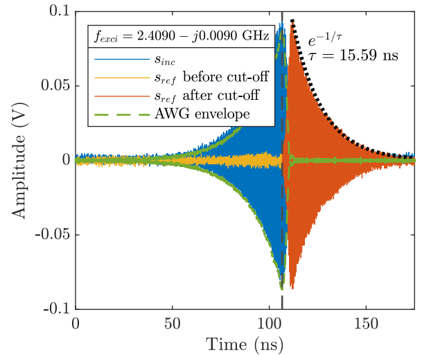
FIG. 7: Observation of a zero of the S-matrix of our cavity through our practical set-up.
