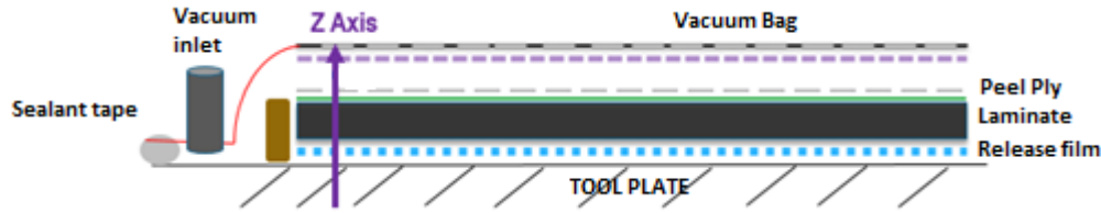
FIGURE 3. Laminating configuration and ancillary products used for manufacturing samples
