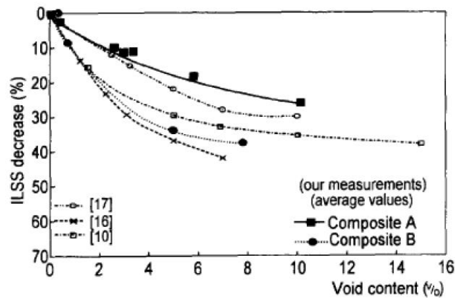
FIGURE 2. Interlaminar Shear Strength (ILSS) as a function of void content 6
