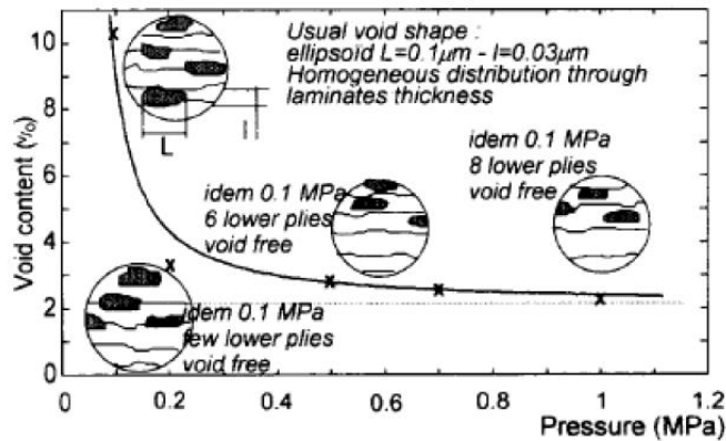
FIGURE 1. Void content as a function of pressure applied during process 6
