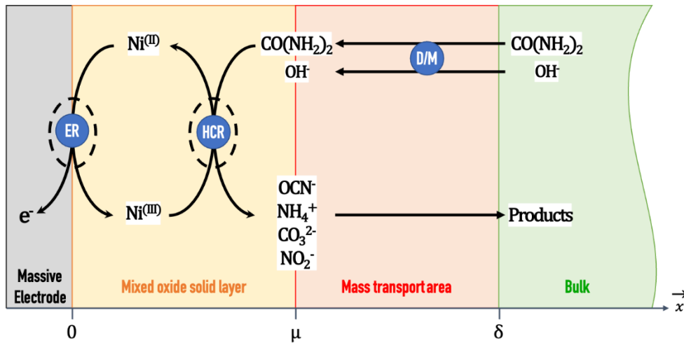
Fig. 3. Schematic representation of the indirect oxidation of the urea, by the electromediation of the system \text{Ni}(\text{OH})_2/\text{NiOOH} operating on the surface of a massive nickel anode, and in presence of alkaline medium. ER, HCR, and D/M indicate respectively the locations where the \text{NiOOH} electrogeneration reaction, the heterogeneous catalytic reaction and the mass transport (limited by the diffusion) take place.
