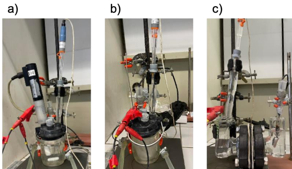
Fig. B.1 Experimental set-ups for i-E plot and electrolysis of urea alkaline solution.
