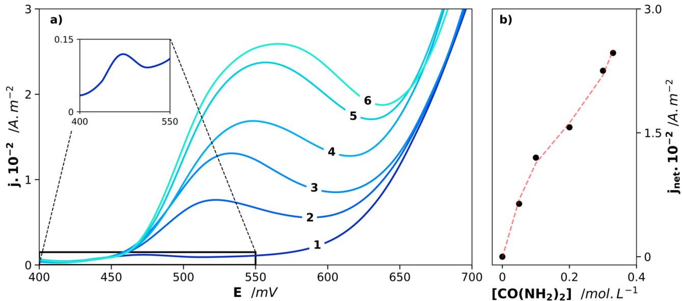
Fig. 2. Effect of the urea concentration a) on the shape of voltammograms obtained on nickel RDE without agitation. [KOH] = 1 mol.L -1 ; v = 1.36 mV.s -1 ; T = 298 °K, S = 3.14 mm 2 . The urea concentration used was 0 mol.L -1 (1), 0.05 mol.L -1 (2), 0.1 mol.L -1 (3), 0.2 mol.L -1 (4), 0.3 mol.L -1 (5) and 0.33 mol.L -1 (6). Fig. 2-b) shows the evolution of the intensity of the oxidation peak as a function of the urea concentration.
