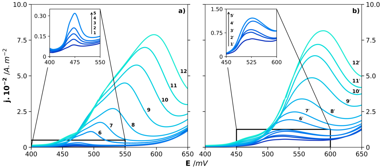
Fig. 4. Effect of potential scan rate on the voltammograms obtained without agitation on nickel electrode immersed into a) in 1 \text{ mol} \cdot \text{L}^{-1} KOH solution b) in 1 \text{ mol} \cdot \text{L}^{-1} KOH containing 0.05 \text{ mol} \cdot \text{L}^{-1} of urea. The scan rate used was 0.58 \text{ mV} \cdot \text{s}^{-1} (1-1'), 1.36 \text{ mV} \cdot \text{s}^{-1} (2-2'), 2.16 \text{ mV} \cdot \text{s}^{-1} (3-3'), 2.91 \text{ mV} \cdot \text{s}^{-1} (4-4'), 5 \text{ mV} \cdot \text{s}^{-1} (5-5'), 25 \text{ mV} \cdot \text{s}^{-1} (6-6'), 50 \text{ mV} \cdot \text{s}^{-1} (7-7'), 100 \text{ mV} \cdot \text{s}^{-1} (8-8'), 200 \text{ mV} \cdot \text{s}^{-1} (9-9'), 300 \text{ mV} \cdot \text{s}^{-1} (10-10'), 400 \text{ mV} \cdot \text{s}^{-1} (11-11') and 500 \text{ mV} \cdot \text{s}^{-1} (12-12'). The insets show a zoom in the oxidation peaks at low potential scan rate.
