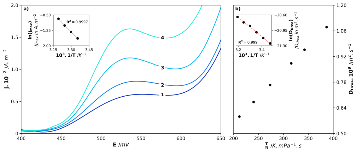
Fig. 9. a) Effect of temperature on the voltammograms obtained at 0.66 \text{ mV}\cdot\text{s}^{-1} , on nickel RDE in a 1 \text{ mol}\cdot\text{L}^{-1} KOH solution containing 0.33 \text{ mol}\cdot\text{L}^{-1} urea. The temperature used was 298 K (1), 303 K (2), 308 K (3) and 313 K (4). \omega = 200 \text{ RPM} . Inset: \ln(j_{\max}) = f(1/T) plotted to determine the activation energy of the global process.
