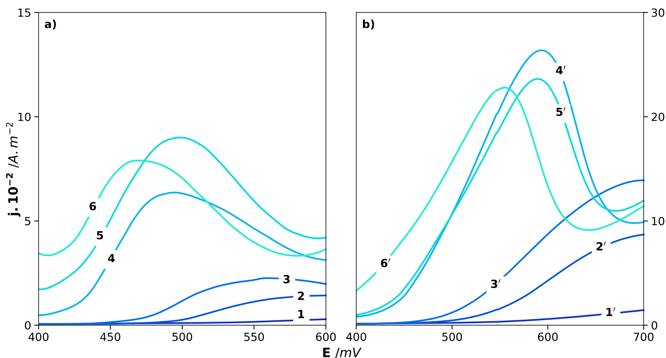
Fig. 7. Effect of KOH concentration by linear voltammogram of nickel RDE in a solution containing 0.33 mol.L -1 urea at a) 1.36 and b) 500 mV.s -1 without agitation at 298 K. The potassium hydroxide concentration used was 0.05 mol.L -1 (1-1'), 0.5 mol.L -1 (2-2'), 1 mol.L -1 (3-3'), 3 mol.L -1 (4-4'), 4 mol.L -1 (5-5') and 5 mol.L -1 (6-6').
