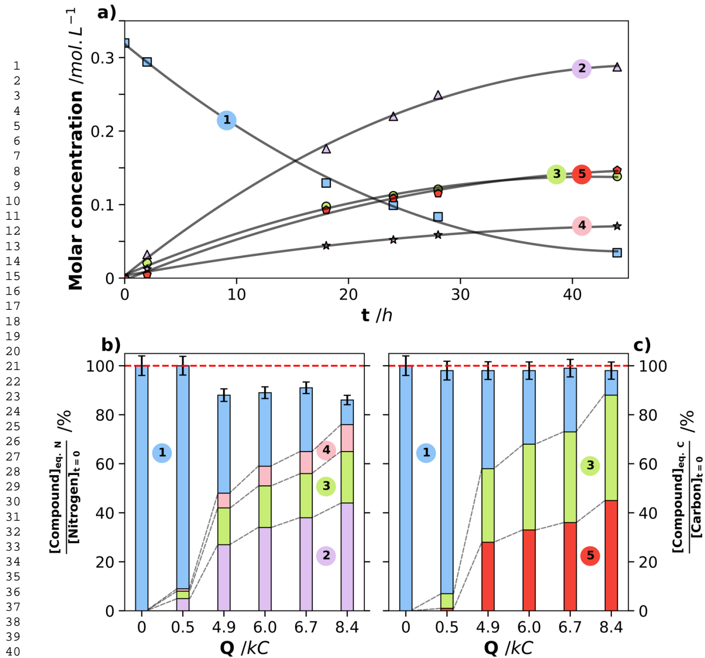
Fig. 11. Results of a typical potentiostatic preparative electrolysis on nickel electrode. S = 4 \text{ cm}^2 ; [\text{KOH}] = 1.5 \text{ mol.L}^{-1} ; [\text{CO}(\text{NH}_2)_2]_{t=0} = 0.33 \text{ mol.L}^{-1} ; E_{\text{applied}} = 550 \text{ mV} ; T = 298 \text{ K} ; V = 50 \text{ mL} . The graph a) shows the molar urea concentration profiles over the electrolysis time, as well as those for the obtained byproducts (the line curves are plotted with the aim of interpolating the concentration behavior, and thus do not correspond to modeling). The error bars in part a) are smaller than the size of labels and evaluated at 4%. The graph b) presents the nitrogen mass balance while the right part c) focuses on the carbon mass balance. The red dotted lines (in b) and c)) show a mass balance of 100%. The error bars represent the total error of the percentages. Labels : ①- \square \text{CO}(\text{NH}_2)_2 , ②- \triangle \text{NH}_4^+ , ③- \circ \text{OCN}^- , ④- \star \text{NO}_2^- and ⑤- \diamond \text{CO}_3^{2-} .
