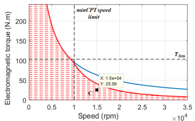
Fig. 11 High-speed operating point marked inside the minCLPT working area
