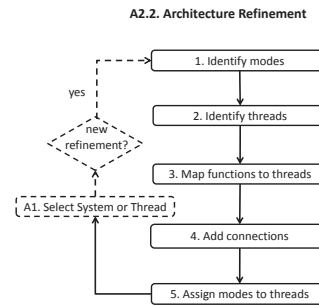
Fig. 3. Refined steps from Architecture Refinement
