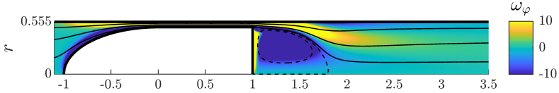
Figure 10: Azimuthal vorticity and streamlines of the base flow in the moving frame attached to the body for L/d = 2 and a/A = 0.81 , Re = 110 .
