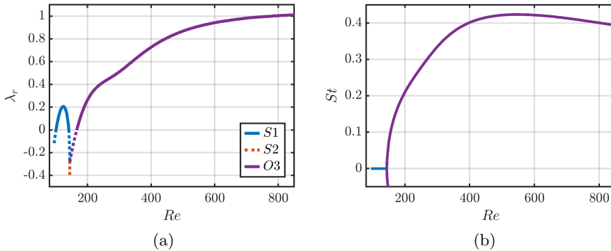
Figure 11: Amplification rate and Strouhal number for the three modes found for L/d = 2 and a/A = 0.81 . The horizontal range of the figure corresponds to Re \in [80 - 850] .
