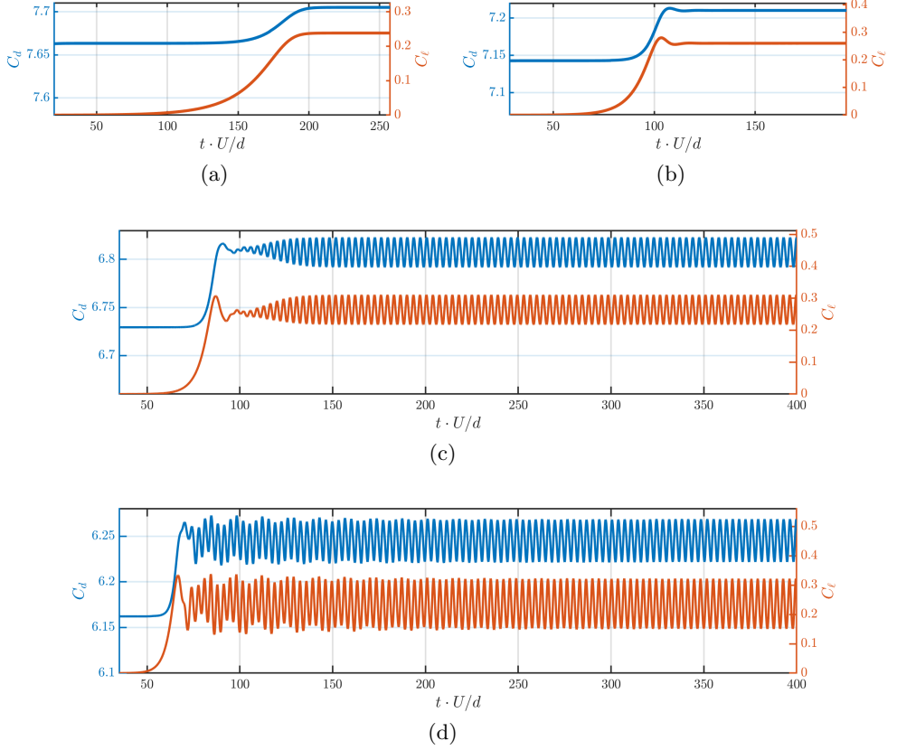
Figure 20: Lift and drag coefficients from DNS simulations ( L/d = 2 and a/A = 0.39 ) versus dimensionless time, for (a) Re = 145 , (b) Re = 160 , (c) Re = 175 and (d) Re = 200 .
