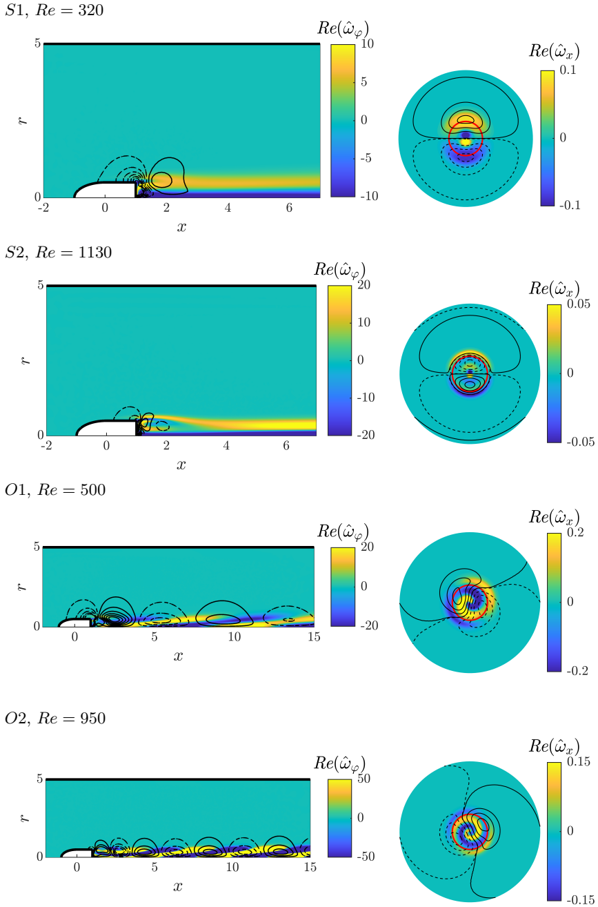
Figure 5: Eigenmodes found for a/A = 0.01 , real parts of the vorticity with iso-levels of pressure. Slices are defined by x = 2 and r \leq 2 .
