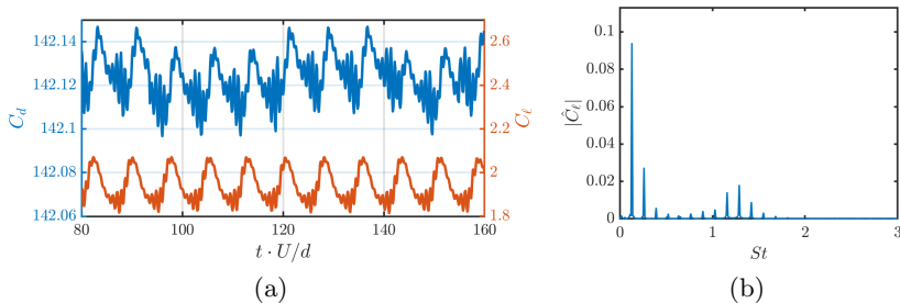
Figure 23: Characterisation of time-dependent forces exerted on body for Re = 150 , a/A = 0.74 : (a) time-history of lift and drag coefficients, and (b) Frequency spectrum of the lift coefficient.
