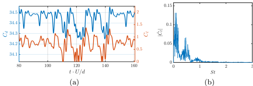
Figure 24: Characterisation of time-dependent forces exerted on body for Re = 150 , a/A = 0.6 : (a) time-history of lift and drag coefficients, and (b) Frequency spectrum of lift coefficient.
