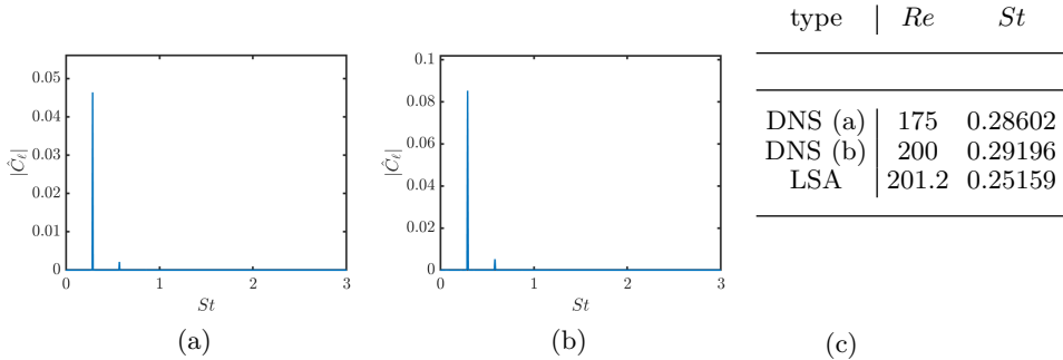
Figure 21: Frequency spectra for DNS case L/d = 2 , a/A = 0.39 , Re = 175 (a) Re = 200 (b) and table of St values of the higher peaks (DNS) with corresponding St_c for LSA (c).
