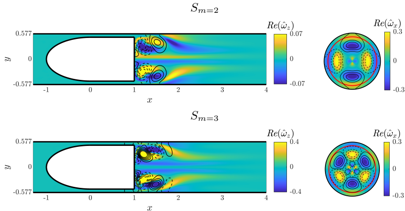
Figure 16: Unstable non-oscillating modes at Re = 200 and a/A = 0.75 . Left: z -component of the vorticity and iso-level of pressure. Right: slice in the transverse plane at x = 2 , streamwise component of the vorticity and iso-levels of pressure, the red circle represents the projection of the base of the blunt body in this plane.
