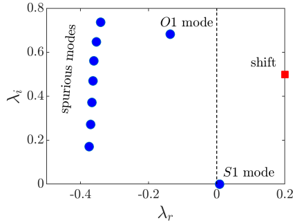
Figure 3: Example of a spectrum found with the shift and invert algorithm ( Re = 320 , L/d=2 , a/A=0.01 ). The 10 eigenvalues closest to the "shift" value indicated in red are computed.
