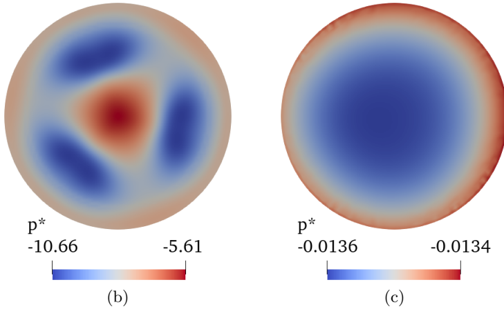
Figure 25: Illustration of the wake for a/A = 0.85 and Re = 150 . Iso-contour of Q-criterion (a), side and rear diagonal views. Slices of the dimensionless pressure p^* = p/(\rho U^2) in the wake of the body, at x/D = 1.2 (b) and at x/D = 9 (c).
