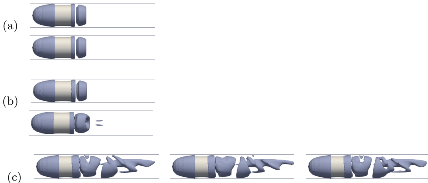
Figure 22: Iso-contour of Q-criterion for moderately confined cases; two perpendicular views are represented for each case. (a) a/A = 0.74 , Re = 100 , (b) a/A = 0.74 , Re = 115 , (c) a/A = 0.74 , Re = 160 . For the last case, instantaneous representations for three different instants are displayed.
