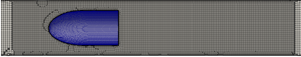
Figure 27: Axial cut-of of the mesh B
