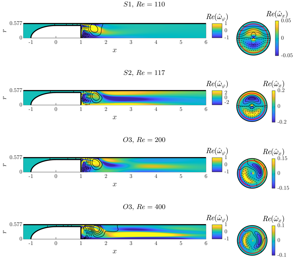
Figure 9: Eigenmodes found for a/A = 0.75 , real parts of the streamwise vorticity with iso-levels of pressure.
