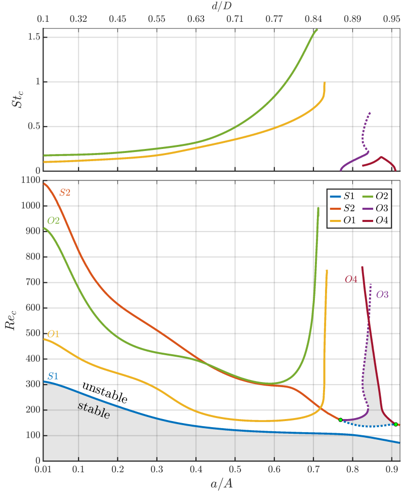
Figure 13: Neutral curves in the Re - a/A plane, and critical Strouhal number as a function of the confinement ratio. The body length is kept constant, L/d = 2 . The dashed portions of the blue and purple curves are part of the neutral curves corresponding to restabilization of the S1 and O3 modes.
