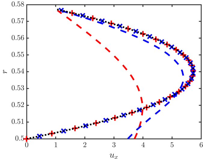
Figure 7: Axial velocity u_x as function to r for Re = 110 (red) and Re = 320 (blue) at locations x = 0.75 (symbols) and x = 1.25 (dashed lines); Comparison with annular Poiseuille solution (black dotted line).
