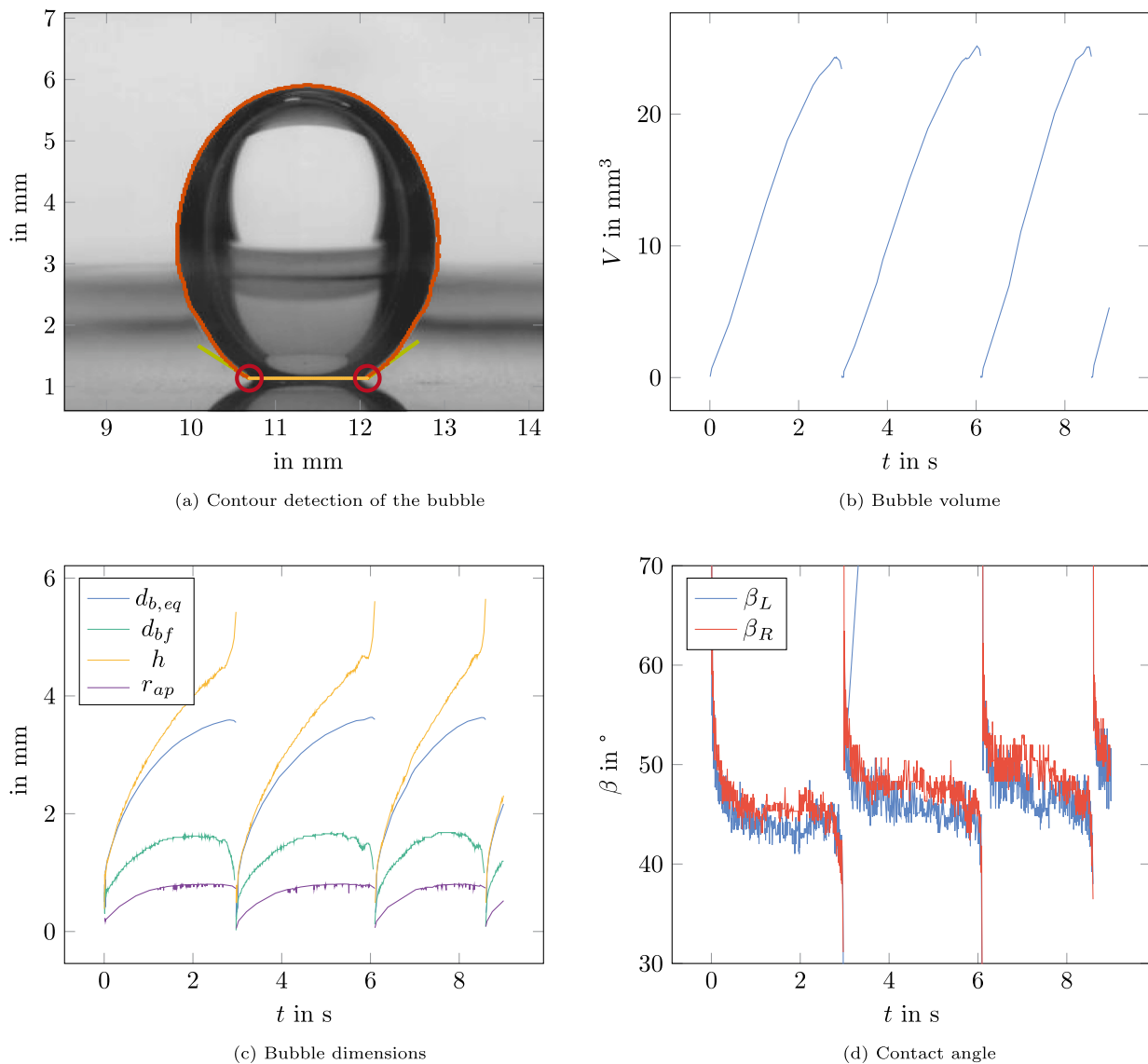
Fig. 21. An example of Matlab code edge detection process (a), bubbles volume (b), bubbles equivalent diameter, foot diameter, height and apex radius (c), left and right contact angles (d). Experimental parameters: p_l = 600 mbar, T_{sub} = 5 K, \dot{q} = 0.75 W cm ^{-2} , t_{wait} = 10 s, E = 2.5 MV m ^{-1} .
