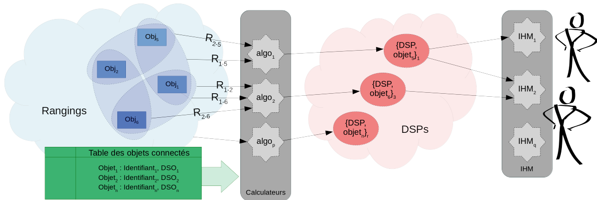
Figure 4.13 – Architecture IDEALI1
