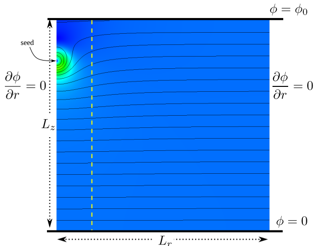
Figure 2: Initial electric field configuration with equipotential lines, where \phi_0 = 18.75 kV and L_z = L_r = 1.25 cm. For the electric potential Neumann zero boundary ( \partial_r \phi = 0 ) conditions are applied at r = 0 (due to symmetry) and at r = 1.25 cm. Neumann zero boundary conditions are implemented for the electron density on all the boundaries. Instead of a needle electrode a positive immobile seed with a Gaussian distribution at (r, z) = (0, 1) cm is included. The dashed white line indicates the radial domain up to 2 mm that is shown in fig. 3, 9, and 17.
