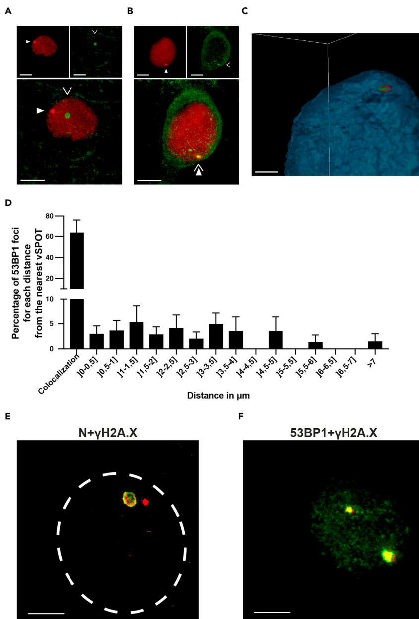
Figure 3. BoDV-1 vSPOT and DSB are strongly colocalized in infected neuronal nuclei
