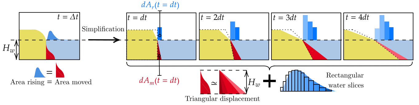
FIG. 11: The morphologies of the slide and wave during formation are simplified based on hypotheses (H3b)-(H6b), and the result is illustrated at successive timesteps, with the same system of symbols as in figure 10.
