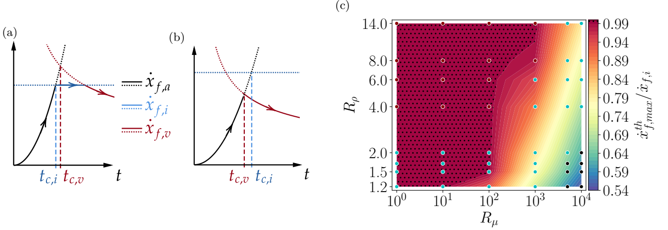
FIG. 7: Transition between regimes (a) in the order acceleration-inertial-viscous for t_{c,i} < t_{c,v} , (b) in the order acceleration-viscous for t_{c,i} > t_{c,v} . For (a) and (b), the three regimes (11)-(12)-(13) are visible respectively in dark, blue and red curves. The curve of every regime is solid when the slide evolves in this regime, and it is in dotted line otherwise. Vertical dashed lines indicate the intersection of the acceleration regime (in dark) with another one. (c) Theoretical value of the ratio \dot{x}_{f,max}^{th} / \dot{x}_{f,i} calculated from the analytical expressions (11)-(13). The dotted region corresponds to unit values of \dot{x}_{f,max}^{th} / \dot{x}_{f,i} .
