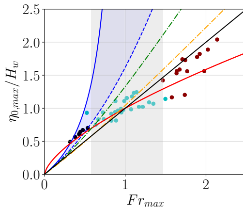
FIG. 12: Comparison of models of wave formation to numerical measurements, at the specific moment t_{max} when the slide front velocity is maximum. Dimensionless wave amplitudes are shown as a function of the measured Froude number Fr_{max} . Bullet points: measurements of \eta_{0,max}/H_w . Rectangular collapse: — equation (25), - - - equation (26). Triangular collapse: — equation (24), — equation (27). Dash-dotted lines correspond to the models from Sarlin et al. [26] for a solitary-like wave (-.-.-) and a bore (-.-.-). The shaded Froude numbers correspond to the region of hydraulic jumps identified in figure 9.
