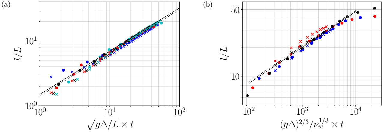
FIG. 15: Test of the numerical methods with experiments from [37]. Numerical results appear in crosses, experimental data as bullet points. (a) Inertial regime of spilling, with colours corresponding to experiments ●9, ●11, ●14, ●18 as numbered in [37], and the regressions — \alpha_1 = 1.5 obtained from experiments and \cdots\cdots\alpha_1 = 1.42 obtained from the associated simulations. (b) Viscous regime of spilling, with colours corresponding to experiments ●19, ●24, ●27 as numbered in [37], and the regressions — \alpha_2 = 1.5 from experiments and \cdots\cdots\alpha_2 = 1.55 from simulations.
