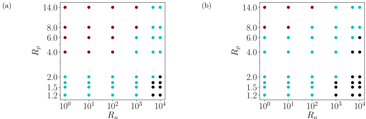
FIG. 3: Maps of the type of wave in (R_\mu, R_\rho) , in the close field (a) and at x = 10W_c (b). Colormap: ● rollers, ● hydraulic jumps, ● solitary-like waves.
