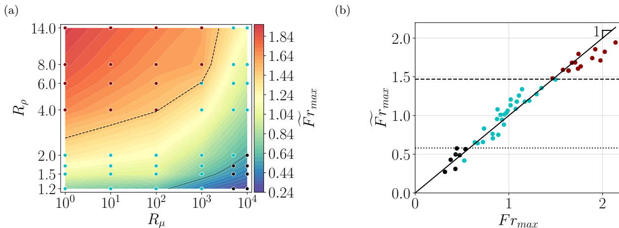
FIG. 9: (a) Map of the predicted maximum Froude number \widetilde{Fr}_{max} . (b) Comparison of Fr_{max} and \widetilde{Fr}_{max} , respectively the measured and predicted maximum Froude numbers. The dispersion of data around the first bisector in solid line is of 11.1%. For both figures, dots are coloured as wave types and the dotted (respectively dashed) line separates hydraulic jumps from solitary-like waves (resp. from rollers).
