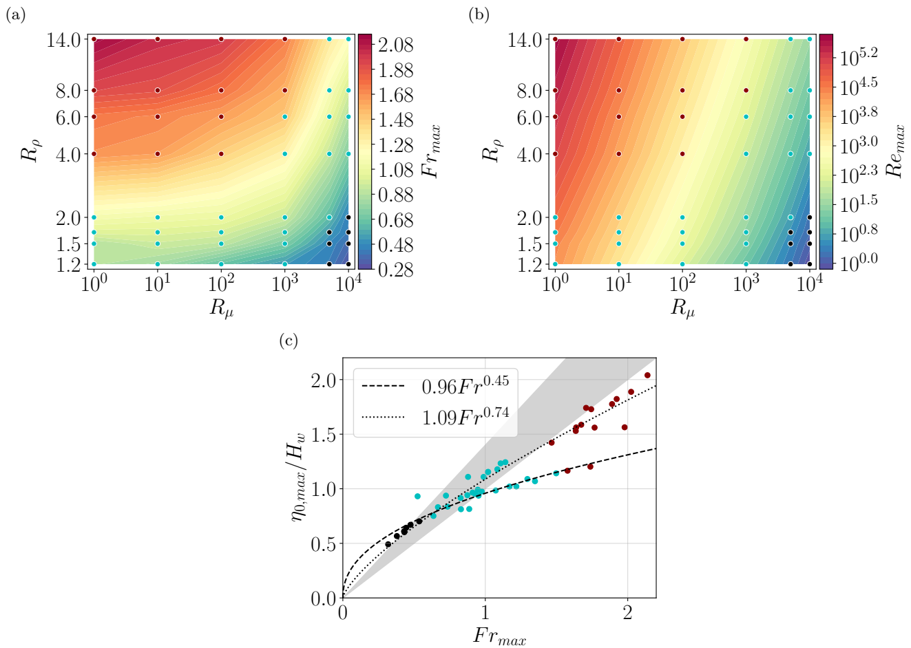
FIG. 6: Maps of Fr_{max} (a) and Re_{max} (b) in (R_\mu, R_\rho) . (c) Evolution of the maximum wave amplitude versus Fr_{max} . The shaded cone corresponds to slopes within the range 1 – 1.4. Two branches are distinguished in the region where \eta_{0,max}/H_w > 1 : those having R_\mu \geq 10^3 (lower branch, dashed curve with a coefficient of correlation r^2 = 0.884 ) and those having R_\mu < 10^3 (upper branch, dotted curve with a coefficient of correlation r^2 = 0.949 ).
