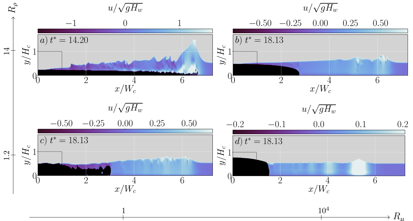
FIG. 2: Waves produced in the four extreme configurations of the parameter space. The layout (see arrows) is such that R_\mu (respectively R_\rho ) increases from left to right (resp. from bottom to top). Air and slide are respectively masked in grey and dark while the horizontal velocity field appears in water. The dimensionless time corresponds to t^* = t\sqrt{g/H_c} . (a): roller (R_\mu, R_\rho) = (1, 14) . (b): hydraulic jump (R_\mu, R_\rho) = (10^4, 14) . (c): hydraulic jump (R_\mu, R_\rho) = (1, 1.2) . (d): solitary-like wave (R_\mu, R_\rho) = (10^4, 1.2) . Dotted lines indicate the initial position of the slide.
