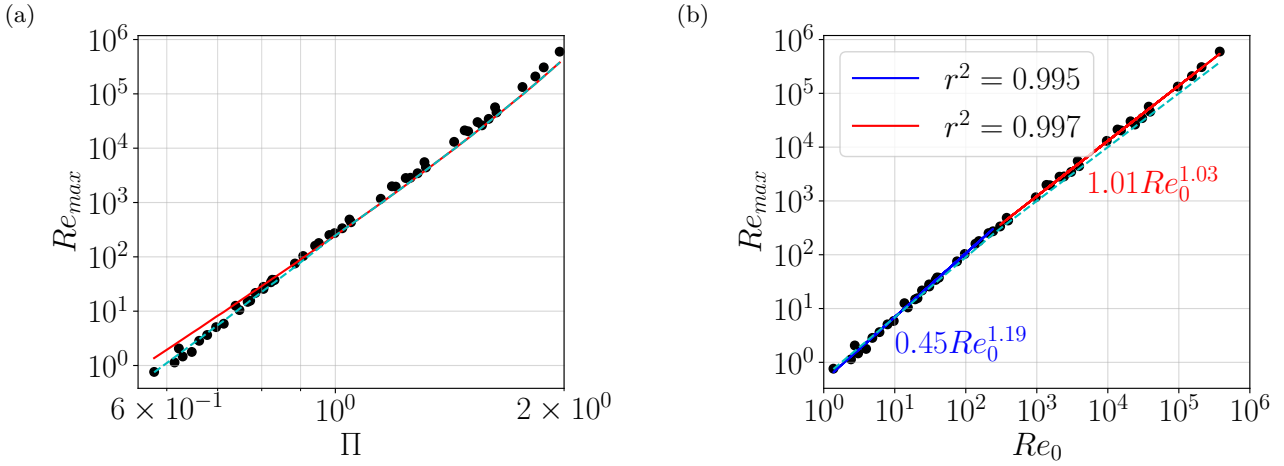
FIG. 8: (a) Correlation between the ratio \Pi = t_{c,v}/t_{c,i} and the following Reynolds numbers: • measurements of Re_{max} , — analytical values of Re_0 from (15), - - - analytical values of Re(\dot{x}_{f,max}^{th}) from (16). (b) Empirical regressions for Re_{max}(Re_0 < Re_{0,c}) and Re_{max}(Re_0 \geq Re_{0,c}) , again with analytical values of Re(\dot{x}_{f,max}^{th}) in dashed cyan line (- - -).
