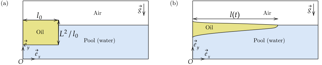
FIG. 14: Representation of the geometry of the problem, (a) initially and (b) at larger times once the oil slick propagates.
