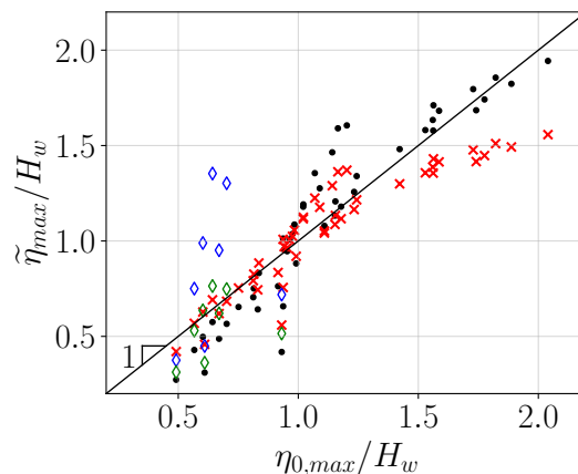
FIG. 13: Assessment of the capacity of previous equations (in ordinate) to predict \eta_{0,max}/H_w from initial conditions. Rectangular collapse: \diamond equation (25), \diamond equation (26). Triangular collapse: \bullet equation (24), \times equation (27).
