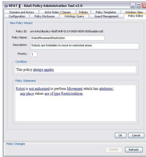
Fig. 4: Example of KAoS policy (from [19])
