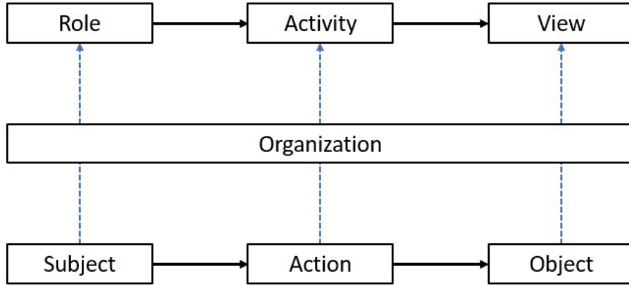
Fig. 3: OrBAC abstraction
