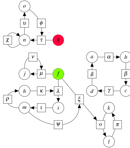
Figure 8: Partial Hard RAF with input (the sources of the attacks \tau , \mu , \lambda and \xi are the inputs, given with their labelling issued to \mathcal{L}_{gr} )
