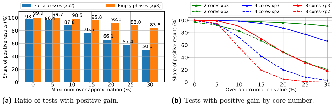
■ Figure 6 Experiments with accesses in each phase ( xp2 ) and with phases without accesses ( xp3 ).
