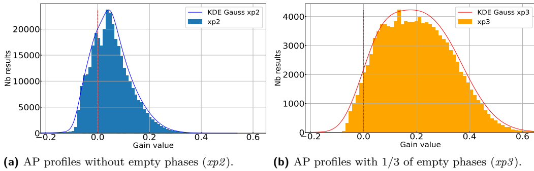
■ Figure 7 Gain distribution for AP profiles with 0 to 10% of over-approximation.
