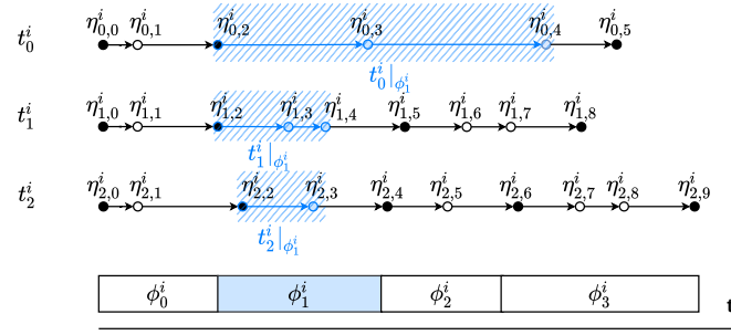
■ Figure 2 Restrictions of traces t_0^i , t_1^i and t_2^i to phase \phi_1^i .
