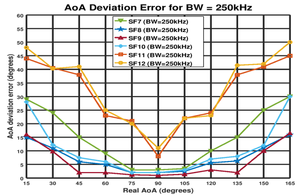
Fig. 5. AoA accuracy for BW = 250 kHz
