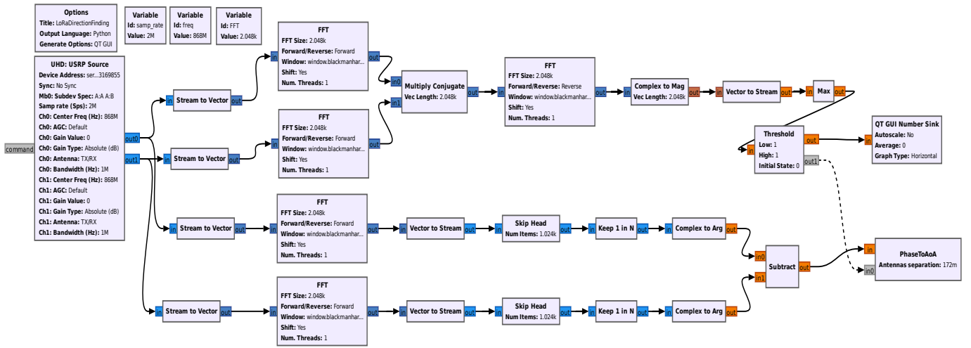
Fig. 3. USRP B210 direction finding system using Autocorrelation - GNU Radio Flowgraph
