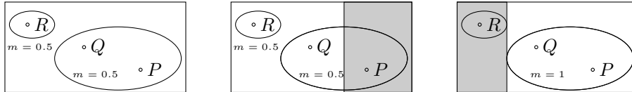
Figure 2: Prior knowledge (left) and revised knowledge given \{Q, R\} (center) and given \{P, Q\} (right). White and gray areas denote possible and impossible events – circles denote focal elements.
