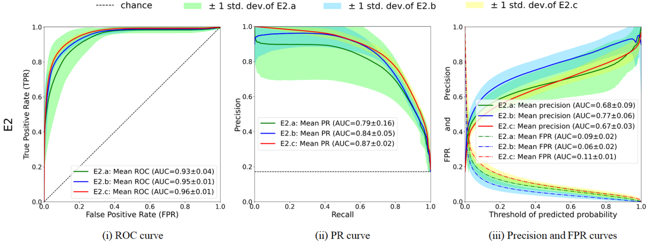
Fig. 9: Over-representation of negative classes \neg\mathbb{C} reduces false positives (hypothesis H2). Mean curves with standard deviation for experiment settings E2.a (for balanced distribution in the training set, green), E2.b (for over-represented \neg\mathbb{C} , blue) and E2.c (for over-represented \mathbb{C} , red). Experiments test H2 in the case of E2, and every example belongs to a single-label category. Same notations as in Figure 7.
