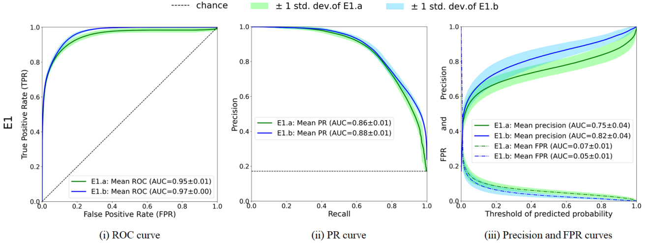
Fig. 7: Natural distribution (E1.b) is better than balanced distribution (E1.a) ( \neg H1 ). Mean curves for (i) the ROC curve, (ii) the PR curve, and (iii) the precision and FPR curves. Sub-figures are obtained for 10 runs for balanced distribution (E1.a, lines in green) and for natural over-representation of \odot distribution (E1.b, lines in blue). The standard deviation is represented by green/blue colored shading. MLNTO data have been used.
