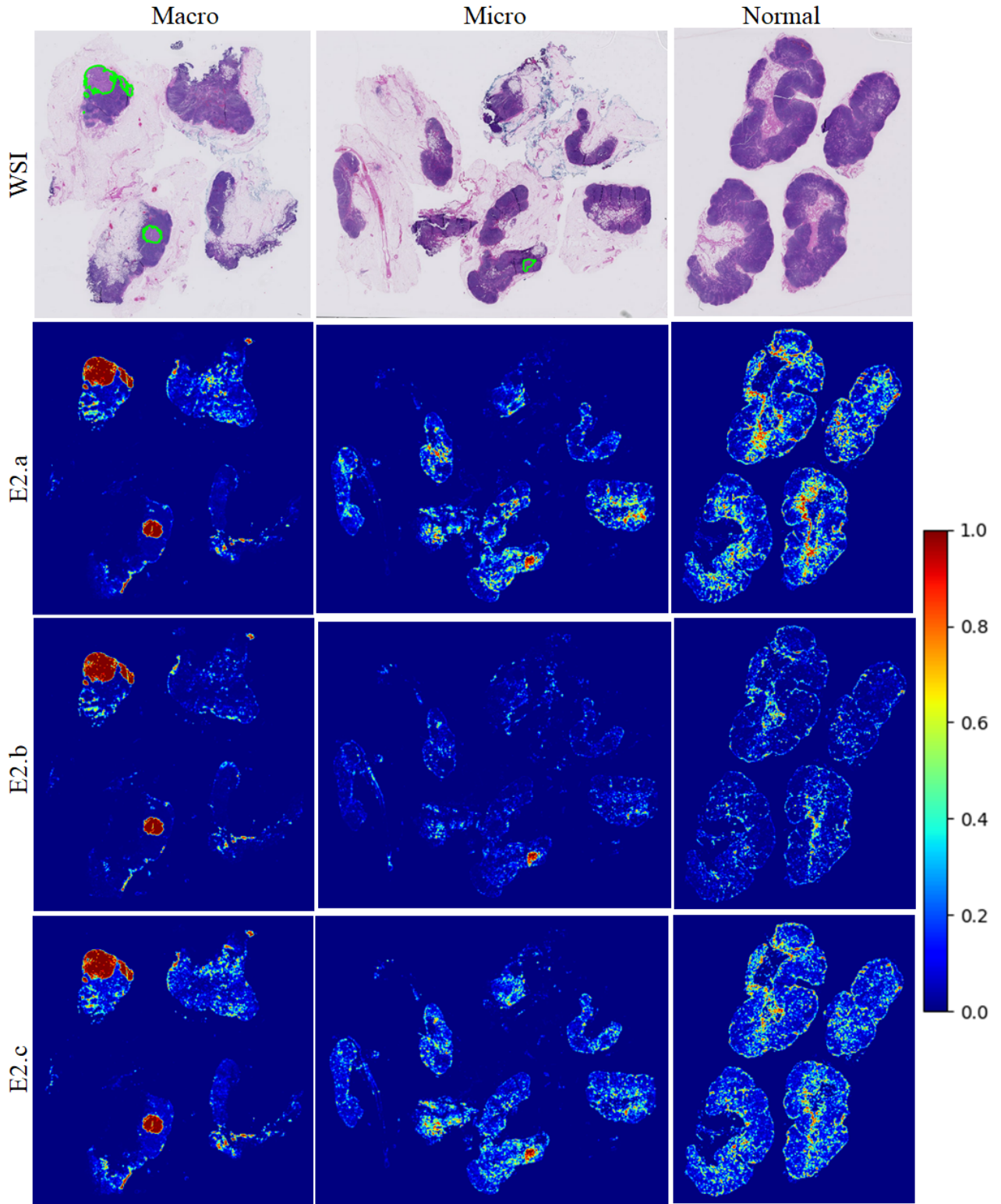
Fig. 16: Illustrative examples for \neg\mathbb{C} -biased training (E2.b) produces the smallest number of FPs (H2). Example heatmaps of class \mathbb{C} generated by the experiments E2.a (for balanced distribution), E2.b (for over-represented \neg\mathbb{C} ) and E2.c (for over-represented \mathbb{C} ) for WSIs with macro-metastasis, micro-metastasis and normal tissue from the CAMELYON16 test set. Here, in the WSIs, the regions inside the green contours are ground-truth annotations for class \mathbb{C} .
