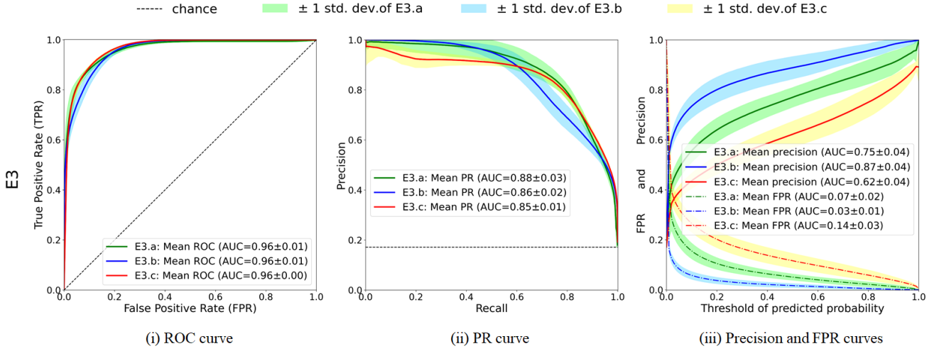
Fig. 12: Multi-label examples give extra advantages over single-label examples (H3 hypothesis). Mean curves with standard deviation using E3 settings (Table 4) where there are multi-label examples: E3.a (for balanced distribution in the training set, green), E3.b (for over-represented \neg\mathbb{C} , blue) and E3.c (for over-represented \mathbb{C} , red) and using the same notations as in Figure 9.
