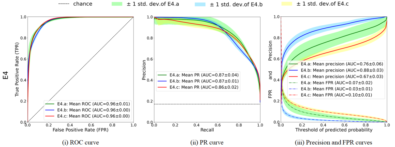
Fig. 13: Non-ROI data are useful (H4 hypothesis). Mean curves with standard deviation using E4 settings (Table 5) where \mathbb{O} examples replace some \mathbb{C} examples and some \neg\mathbb{C} examples: E4.a (for balanced distribution in the training set, green), E4.b (for over-represented \neg\mathbb{C} , blue) and E4.c (for over-represented \mathbb{C} , red) and using the same notation as in previous figures.
