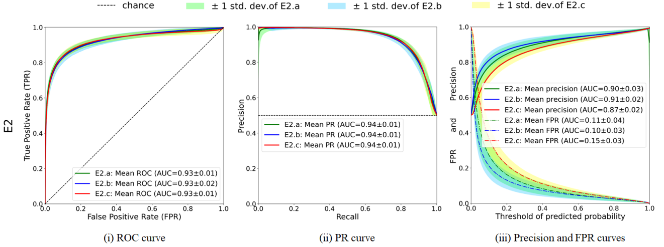
Fig. 14: Over-representing the negative class \neg C reduces false positives - on PCam. Mean curves with standard deviation (std. dev.) of experiments for balanced distribution (E2.a), for over-represented \neg C (E2.b), and for over-represented C (E2.c) on PCam.
