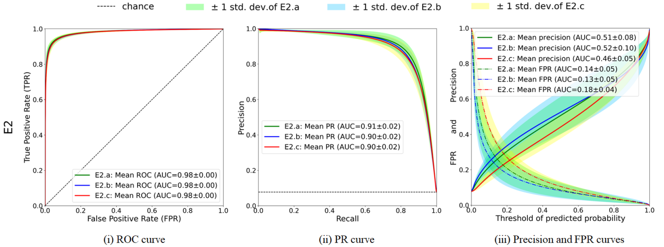
Fig. 15: Over-representing the negative class \neg C reduces false positives - on CAMELYON16. Mean curves with standard deviation (std. dev.) of experiments E2.a (for balanced distribution), E2.b (for over-represented \neg C ) and E2.c (for over-represented C ) using the same keys as in the other figures. In all the experiments, the models were trained on PCam and tested on CAMELYON16.
