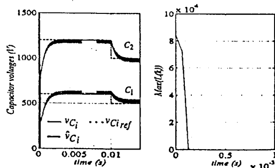
Figure 11. Simulation results using the observer of figure 10.
