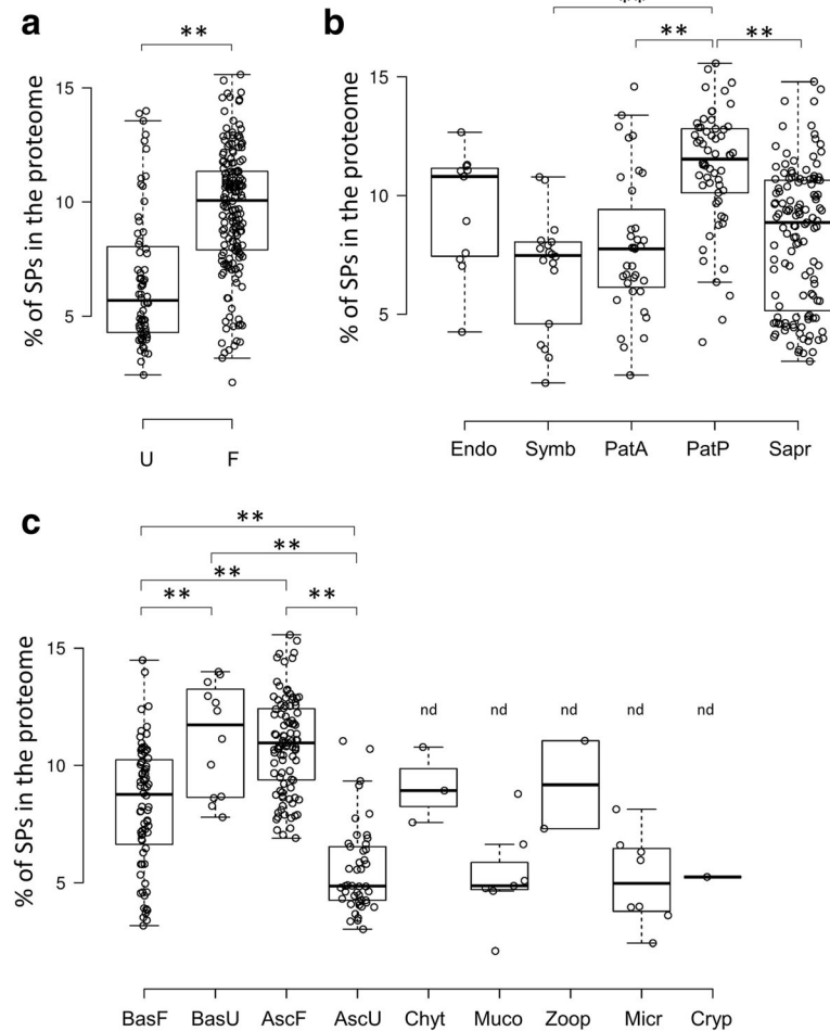
Fig. 1 Proportion of secreted proteins (SPs) in 250 fungal species, with regard to fungal morphology (a), lifestyle (b) and lineage (c). U: yeasts, yeast-like and unicellular fungi, F: filamentous fungi, Endo: endophytes, Symb: symbionts, PatP: plant pathogens, PatA: animal pathogens, Sapr: saprotrophs, BasF: filamentous Basidiomycota, BasU: yeast, yeast-like and unicellular Basidiomycota, AscF: filamentous Ascomycota, AscU: yeast, yeast-like and unicellular Ascomycota, Chyt: Chytridiomycota, Muco: Mucoromycota, Zoop: Zoopagomycota, Micr: Microsporidia, Cryp: Cryptomycota. Statistical analysis was performed with one-way analysis of variance with post-hoc Tukey HSD test; **: p < 0.01 . nd: fungal phylum for which statistical comparisons were not performed
