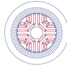
Fig. 1. Transversal section of the PMA-SynRM
