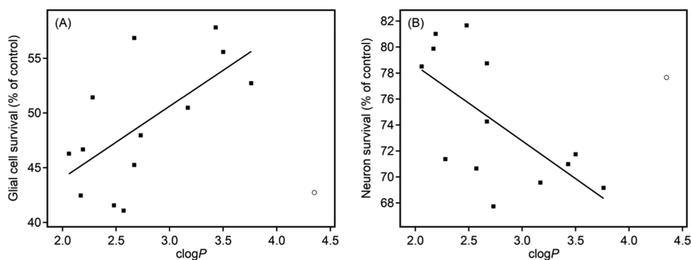
Figure 7. Correlation of octanol–water partition coefficient ( c \log P ) of the nitrones with their protective effect at 10 \mu\text{M} on (A) glial cells challenged by {}^t\text{BuOOH} ( R^2 = 0.41 ) and (B) primary cortical neurons injured by glutamate ( R^2 = 0.42 ), excluding the outlier 4-Ph-PBN marked as \circ .
