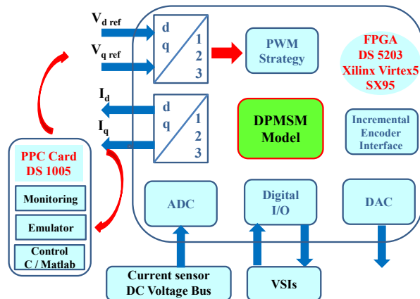
Fig. 3: Task repartition of Real Time Control implemented on FPGA and PPC board.
