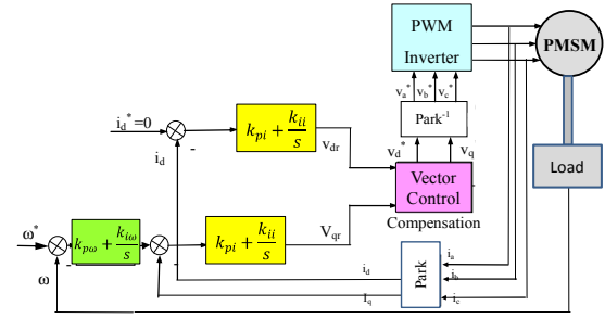
Fig. 2: Diagram of Vector Control of each PMSM
